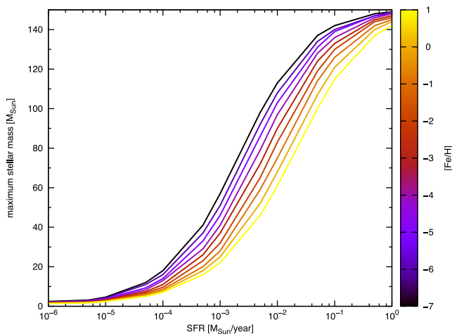
Figure 2. This figure shows how the maximum stellar mass (on the y-axis) varies as a function of the SFR (on the x-axis) and as a function of the [Fe/H] abundance (colour-coding: from -7 dex up to 1 dex). Increasing the [Fe/H] abundance has an opposite effect on m_{\text{max}} with respect to the increasing of the SFR.
