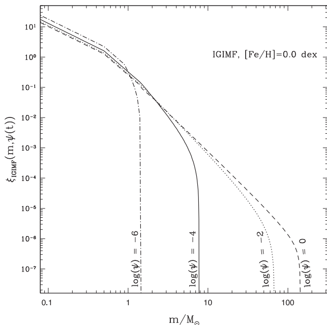
Figure 1. In this figure, we show the predicted IGIMF, \xi_{\text{IGIMF}} , as a function of the stellar mass m in the case of solar iron abundance and for various SFRs: from \psi(t) = 10^{-6} \text{ M}_{\odot} \text{ yr}^{-1} up to \psi(t) = 1 \text{ M}_{\odot} \text{ yr}^{-1} . The net effect of lowering the SFR is to truncate the IGIMF towards lower stellar masses.
