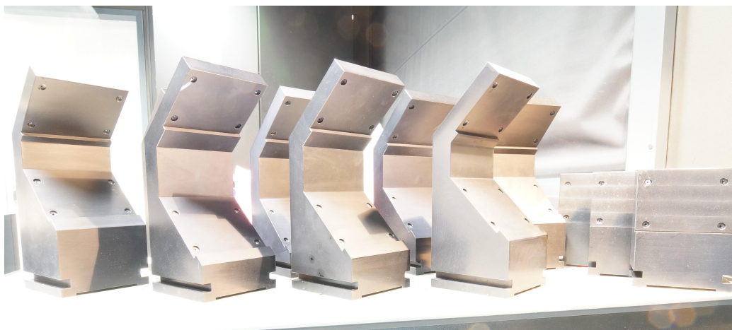
Figure 3: the measurement setup is made possible by fabrication of the precision mirror mounts employing wire-electro discharge machining. This technique easily excels the required tolerances of better than \pm 0.05 \text{ mm} and angularly better than \pm 0.03^\circ .
