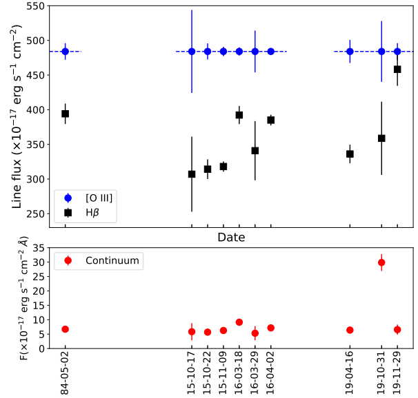
Fig. 6. Variability measured in the continuum flux density and in the H\beta line flux. The blue circles represent the [\text{O III}]\lambda 5007 flux, which was forced to be the same in all spectra. The black squares represent the flux of H\beta , and the red circles in the bottom panel represent the continuum flux.
