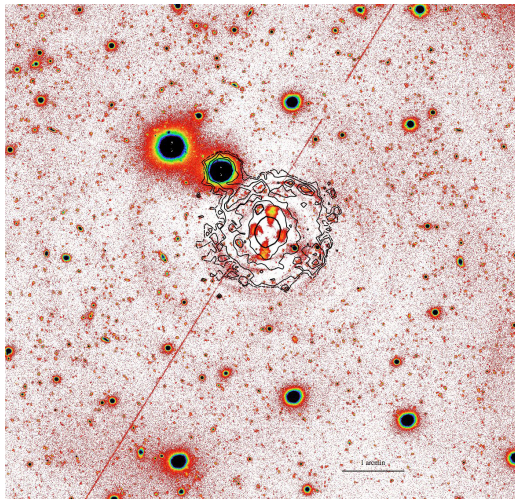
Figure 7. Residual image ( 8/30 \times 7/95 ) from VST g band of NGC 1533 inner region with the contours (levels are 25.26 (bold), 25.85, 26.10, 26.29, 26.41 (dashed) mag arcsec ^{-2} ) obtained from the W2 filter image Swift -UVOT (Rampazzo et al. 2017).
