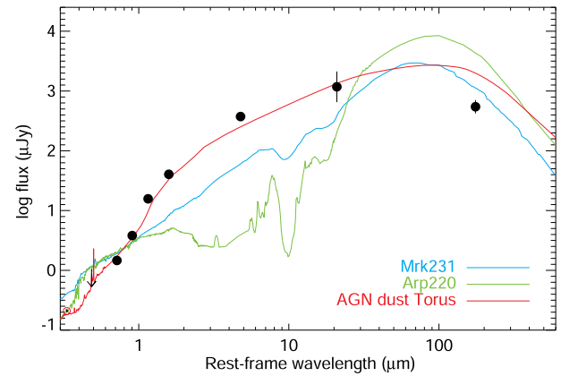
Right: Overlay of the observed data (black) with the SED templates 61 of the AGN-dominated local ULIRG (Mrk 231), the extreme local starburst ULIRG (Arp 220), and the AGN dust torus model at redshift z = 3.965 .
