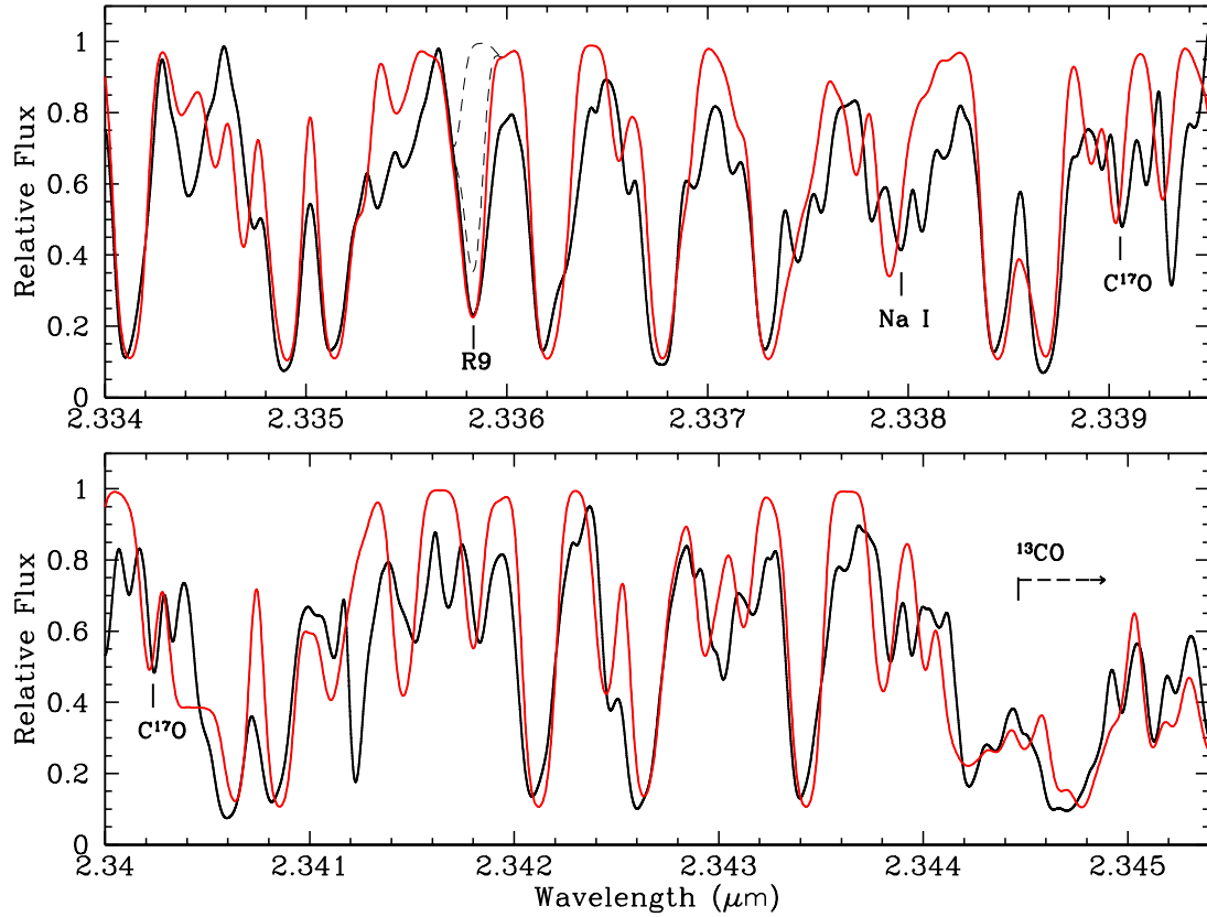
Fig. 1. Comparison between observed (thick black line) and theoretical spectra for the SC-type star R Cmi around the spectral region of the R9(1-0) HF line. Top panel: continuous red line corresponds to the best fit ( \log \epsilon(\text{F}) = 4.9 ) and black dashed lines are synthetic spectra computed with no F and \log \epsilon(\text{F}) = 4.2 , respectively. The R9 HF, Na I and \text{C}^{17}\text{O} lines at \sim 2.3358 , 2.3380 and 2.3395 \mu\text{m} , respectively are marked. Note that the R9 line is blended to the left with a \text{C}^{17}\text{O} line (not marked in the figure). Bottom panel: the same as in top panel showing another \text{C}^{17}\text{O} feature used (among others) to derived the ^{16}\text{O}/^{17}\text{O} ratio, and the head of the ^{13}\text{CO} molecular band from which the ^{12}\text{C}/^{13}\text{C} ratio was derived in some stars (see text).
