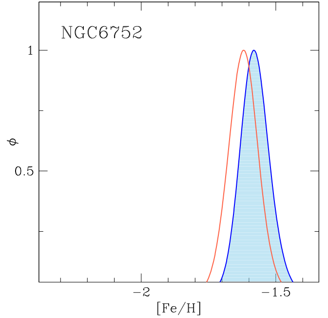
Figure 6. Generalized histograms for [\text{Fe I}/\text{H}] and [\text{Fe II}/\text{H}] (same colors of Figure 2) for a sample of 14 RGB stars in the GC NGC 6752. The analysis has been performed adopting spectroscopic T_{\text{eff}} and photometric \log g , the same method used for the right panel of Figure 2.
