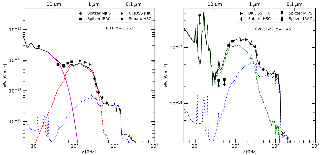
Figure 5. Optical/IR SEDs of RB1 (left) and CVB13-22 (right), the two possible counterparts to the NuSTAR detection in the UDS field. The circular data point is Spitzer MIPS, the square points refer to Spitzer IRAC, the rightward triangles to UKIDSS in the JHK bands, and the diamonds to Subaru HSC in the g , r , i , z , Y bands. The optical-IR part of the SED is fitted with an AGN (solid violet), passive (dashed red), late-type (dotted-dashed green) and star-forming (dotted blue) templates. Upper limits are labeled as downward arrows and have been estimated considering the minimum flux of the sources detected by one instrument in the surroundings of the target. While the AGN component in the SED in RB1 is heavily reddened ( E(B - V) \sim 6.2 ), giving support to the classification of obscured (possibly CT) AGN, the same component in CVB13-22 is not required by the fit.
