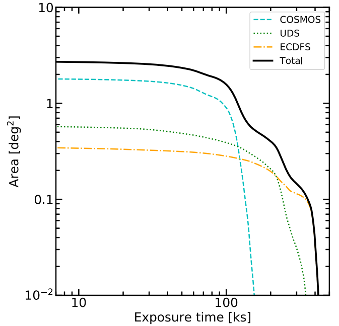
Figure 1. Area as a function of FPMA+FPMB exposure for the three field considered in this work (COSMOS, dashed cyan; UDS, dotted green; ECDFS, dot-dashed orange). The summed area curve is shown as the thick black line, for a total area of 2.74 deg 2 .
