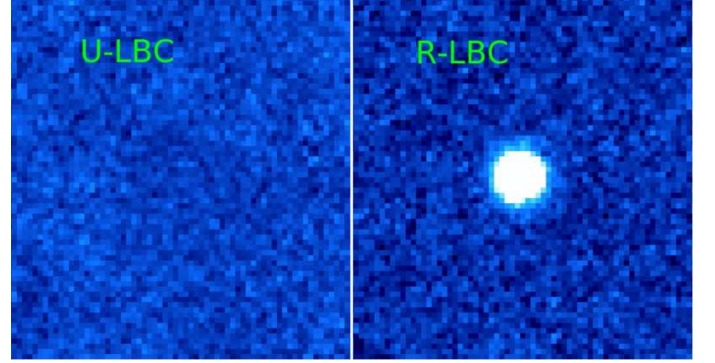
Fig. 5. The stack of the 37 galaxies with 3.27 < z_{\text{spec}} < 3.40 in the U (left) and R bands (right) for the VUDS-LBC/COSMOS, Q0933, and Q1623 fields. Other objects detected in the R band but not associated with the galaxies at z \sim 3.3 (at the center of the FITS thumbnail) have been masked both in the U and in the R band image using the segmentation map derived from the R band. The size of each image is 14 \text{ arcsec} by 14 \text{ arcsec} .
