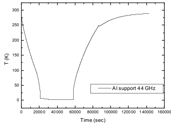
Fig. 33 Cooldown and warmup data of the 8 th cycle for the 44 GHz QM reference load
