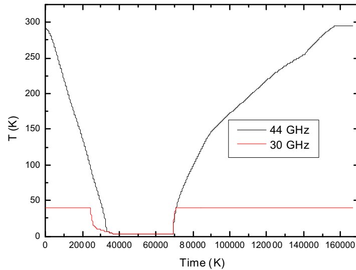
Fig. 38 Cooldown and warmup data for the cycle 12 (13) of the 30 (44) GHz QM reference load
