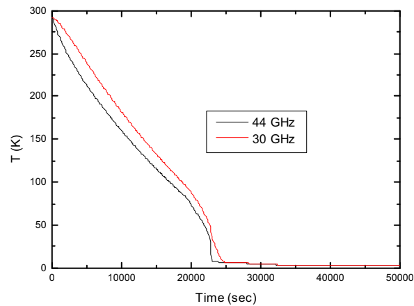
Fig. 31 Cooldown data for the 6 th cycle
