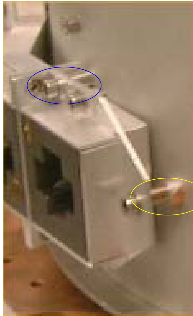
Fig. 5 The sample is mounted on the shield by means of six stainless steel screws and washers (blue line). The lateral fixation is fitted to the cylindrical wall by means of copper adaptors (yellow line).
