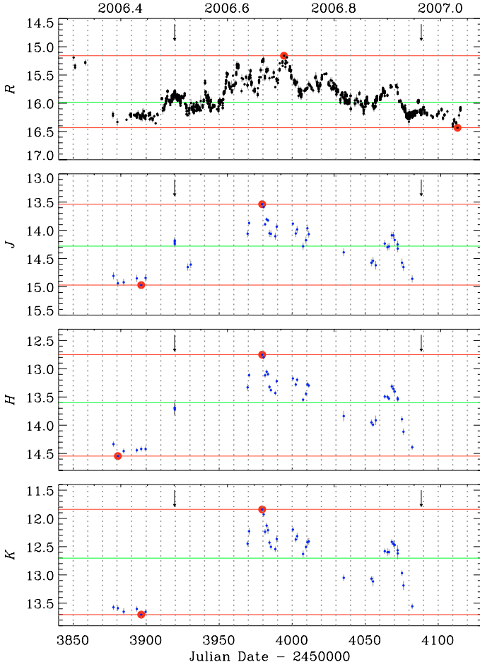
Fig. 2. R -band (top panel) and JHK light curves of 3C 454.3 from May 2006 to January 2007. All near-infrared data are from Campo Imperatore. Maximum and minimum (red lines) as well as average (green lines) brightness levels are indicated. Arrows mark the times of the XMM-Newton pointings of July and December 2006.
