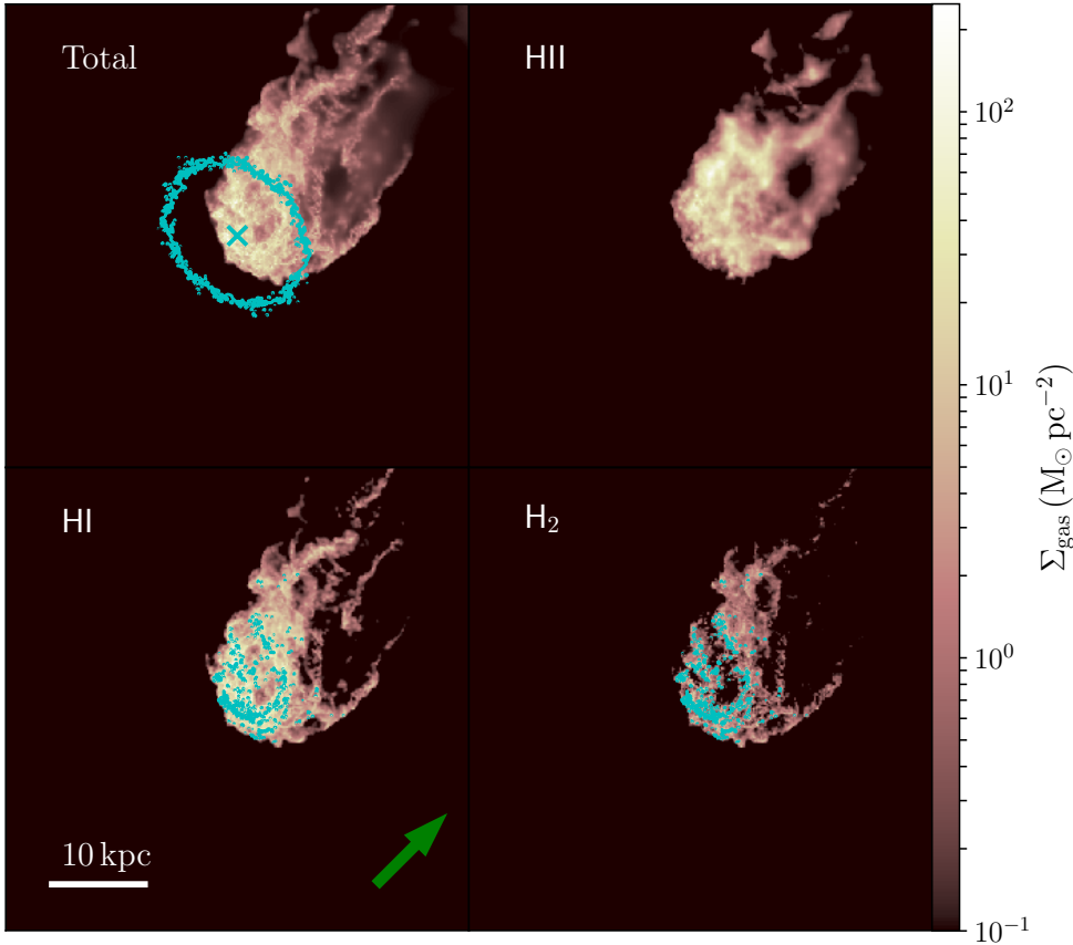
Fig. 17. Two-dimensional distribution of the total (HI, H 2 , HII, He, and metals; upper left panel ), ionised ( upper right ), atomic ( lower left ), and molecular ( lower right ) gas components of the simulated galaxy undergoing a wind of 2000 km s -1 , 150 Myr after the beginning of the interaction. The model galaxy is orientated as IC 3476 on the plane of the sky. The cyan cross in the upper left panel shows the stellar centre, the contours the stellar disc, while those in the lower panels show the distribution of the star-forming regions. The green arrow indicates the direction of the wind.
