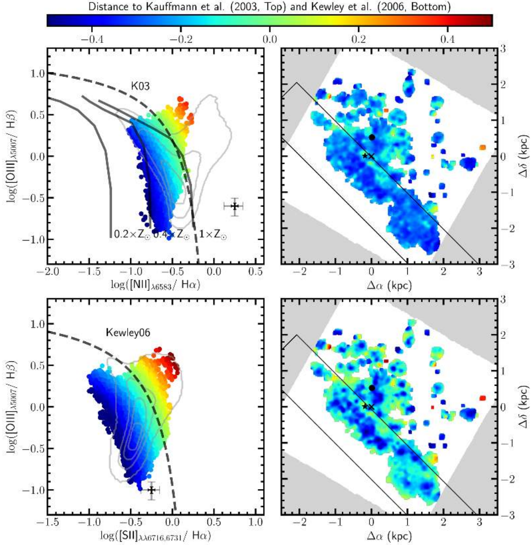
Fig. 10. Left: [OIII]/H \beta vs. [NII]/H \alpha ( upper ) and [OIII]/H \beta vs. [SII]/H \alpha ( lower ) BPT diagrams for emission lines with an S/N > 5 . The dashed curves separate AGN from HII regions (Kauffmann et al. 2003; Kewley et al. 2001, 2006). Data are colour coded according to their minimum distance from these curves. The black and grey crosses indicate the typical error on the data for lines with S/N \approx 15 and S/N \approx 5 , respectively. The grey contours show the distribution of a random sample of nuclear spectra of SDSS galaxies in the redshift range 0.01–0.1 and stellar masses 10^9 \leq M_{\text{star}} \leq 10^{11} M_{\odot} . The thick solid lines in the upper left panel show three different photo-ionisation models at different metallicities (0.2, 0.4, 1 Z_{\odot} ; Kewley et al. 2001). Right: map of the spaxel distribution colour-coded according to their position in the BPT diagram. The cross, star, and filled circle show the position of the photometric, stellar and gas kinematical centres, respectively. The black rectangle indicates the front region of the galaxy (see Fig. 4).
