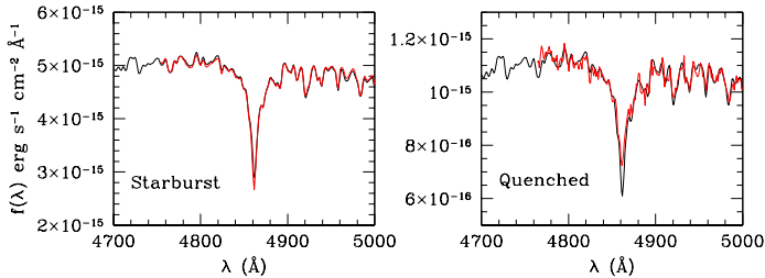
Fig. 12. Best model fit of the stellar continuum obtained with CIGALE (black) is compared to the MUSE spectrum (red) in the H\beta line after the emission is removed using GANDALF for the starburst (left) and quenched (right) regions. The best model has been scaled on the Y-axis to match the observed spectrum.
