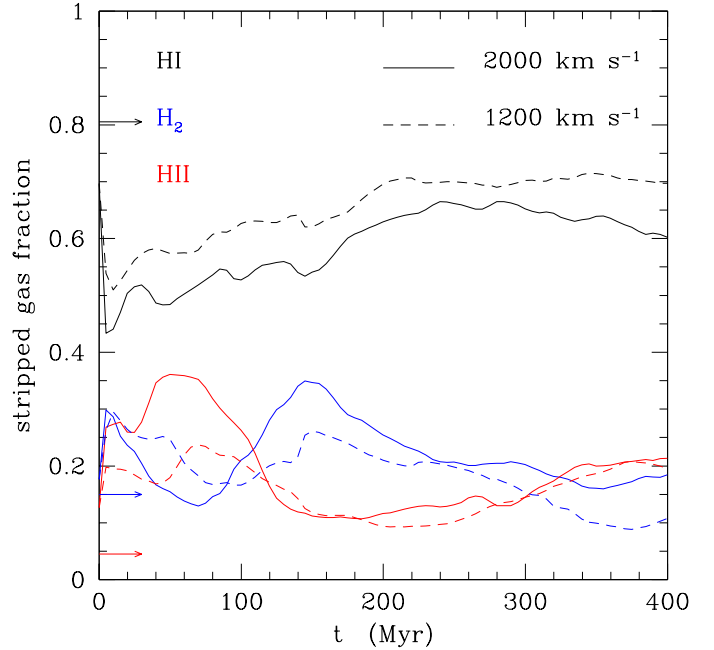
Fig. 20. Variation of the stripped gas fraction within the tail in its different phases (black: H_I ; blue: H_2 ; red: ionised) as a function of time for the simulated galaxy subject to an external wind of 2000 \text{ km s}^{-1} (solid) and 1200 \text{ km s}^{-1} (dashed). The black, blue, and red arrows on the Y-axis indicate for reference the mean H_I , H_2 , and HII gas fractions on the leading side of the unperturbed galaxy disc.
