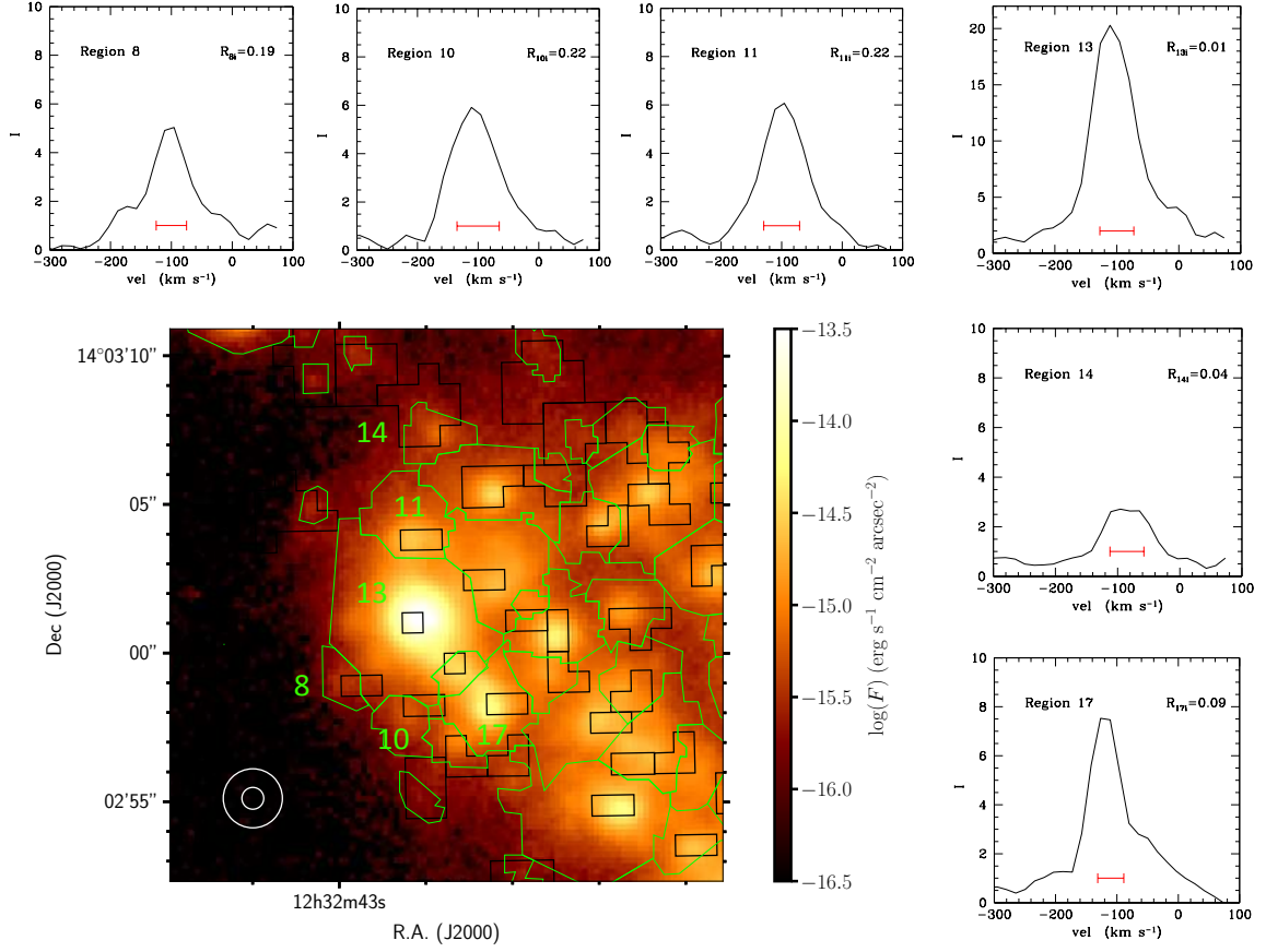
Fig. D.1. Estimate of the kinematical parameters of HII regions in crowded regions. Lower left panel: narrow-band H \alpha image of a crowded region in IC 3476. The boundaries of the individual HII regions identified by the HIIPHOT pipeline are indicated with green contours. The corresponding Voronoi bins in the Fabry-Perot data are indicated with black polygons. The limiting seeing of the VESTIGE and of the Fabry-Perot data are denoted with two concentric circles on the lower left corner of the image. The upper and right-hand panels of the figure show the H \alpha line profiles of the velocity dispersion (in arbitrary units) of the six selected regions indicated in the lower left panel . Of these, regions 10 and 11 do not satisfy the R_{\text{HII}} \leq 0.2 criterion given above, and are thus excluded from the analysis of the kinematical properties of HII regions given in the text, while regions 8, 13, 14, and 17 are included. In each panel, the red horizontal line gives the measured FWHM = 2\sqrt{2\ln 2} \times \sigma , where \sigma is the velocity dispersion.
