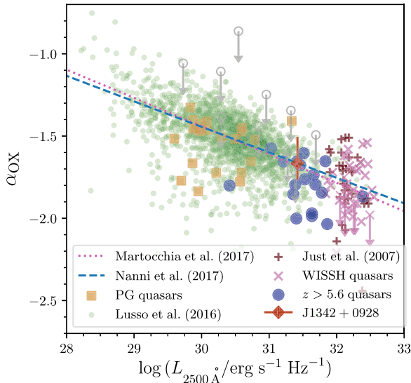
Figure 3. X-ray-to-optical power-law slope ( \alpha_{OX} ) as a function of the rest-frame 2500 Å monochromatic luminosity. The green small circles represent the AGNs from Lusso & Risaliti (2016) with X-ray detections with a signal-to-noise ratio greater than five. We also show the quasars from the Palomar-Green (PG) bright quasar survey (Laor et al. 1994), the hyperluminous SDSS quasars studied by Just et al. (2007), and the WISE /SDSS selected hyperluminous (WISSH) quasar sample (Martocchia et al. 2017) as orange rectangles, maroon plusses, and pink crosses, respectively. The z > 5.6 quasars (circles) and J1342+0928 (red diamond; this work) occupy the locus in between the Lusso & Risaliti (2016) AGNs and the quasar samples of Just et al. (2007) and Martocchia et al. (2017). In the calculation of \alpha_{OX} for the z > 5.6 quasars we used the X-ray fluxes reported by Nanni et al. (2017, 2018) and the rest-frame 2500 Å flux densities, extrapolating the 1450 Å rest-frame magnitudes (see Figure 2), assuming a typical ultraviolet–optical power-law slope of \alpha_U = -0.5 (e.g., Bañados et al. 2015). The dotted and dashed lines are the best-fit relation between \alpha_{OX} and L_{2500\text{Å}} reported by Martocchia et al. (2017) and Nanni et al. (2017), respectively. The uncertainty in \alpha_{OX} for J1342+0928 is dominated by the systematic uncertainty in the X-ray luminosity as it was calculated fixing the power-law photon index to \Gamma = 1.9 (see the text).
