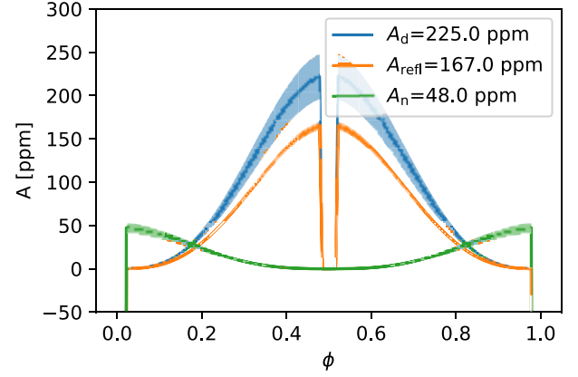
Fig. 3. Upper limits on the reflected PC, dayside thermal PC, and night-side thermal PC for WASP-178 b.
