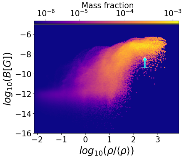
Fig. 13. Phase diagram of the statistical distribution of the magnetic field strength as a function of gas overdensity ( |B| - \rho/\langle\rho\rangle ) from simulations (Vazza et al. 2021). The cyan and the white arrows are the 0.41 and 0.46 nG lower limits on the magnetic field from this work.
