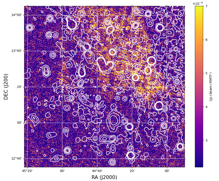
Fig. 4. Slice of the FDF cube at \phi \sim 7.5 rad m -2 showing the Galactic polarised emission detected in the field. Total intensity is overlaid with contours at 4, 20, 40, and 80 \times \text{RMS} taken from Fig. 1.
