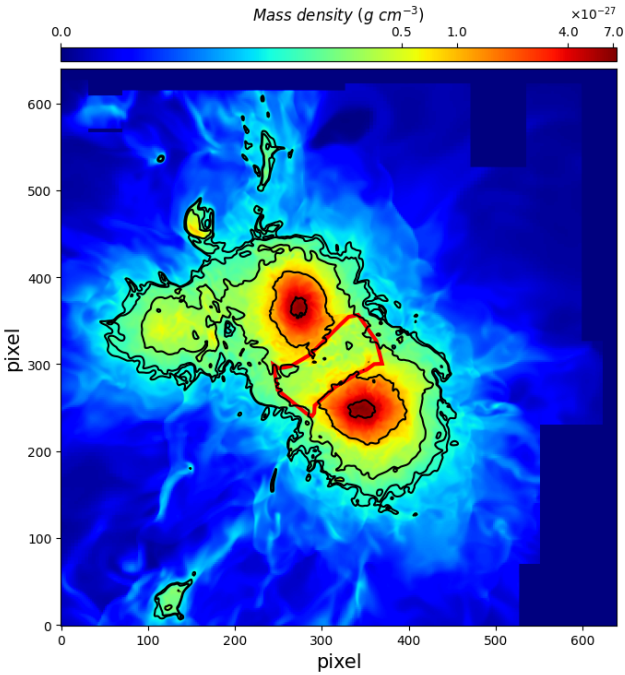
Fig. 10. Central slice of the cube density from simulations. Moving towards the density cube, the average density of the medium initially increases, indicating the presence of the cluster pair, then starts to decrease until reaching zero in the last slice, showing the ending regions of the cluster pair. We therefore selected the central slice of the cube as the best indicator of the density distribution. The density contours are at 1, 1.24, 2.61, 10.3, and 53.5 \times 10^{-28} \text{ g cm}^{-3} . The region selected as the bridge region in the simulation is highlighted in red. Every pixel is \sim 16 \text{ kpc} long.
