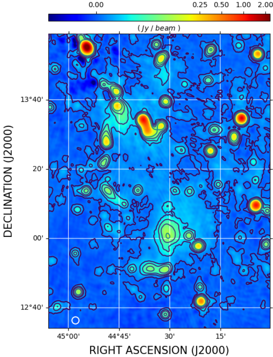
Fig. 1. Image of the A399–A401 pair at 144 MHz. The 107'' \times 107'' restoring beam is shown in white in the bottom left corner. Black contours are drawn at 4, 20, 40, 80, 160, and 320 \times \text{RMS} , where the RMS is 620 \mu\text{Jy beam}^{-1} .
