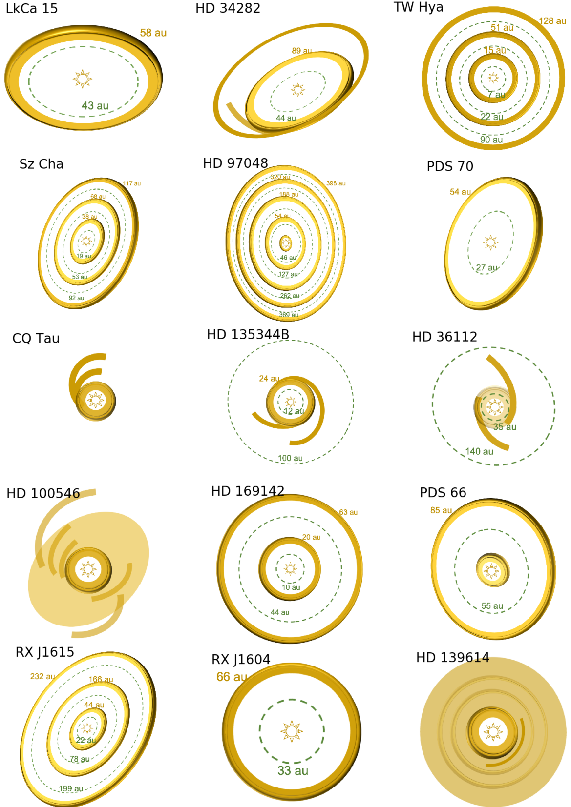
Fig. A.1. Sketch representation of the scattered light appearance of the PPD sample. Included are only the gaps and substructures considered to have been created by perturbors in Sect. 4. The adopted locations of these perturbors are shown as green dashed curves. Scattered-light rings are shown as thick rings, while arms and spiral patterns are shown as flat curled curves. The disks are projected according to their inclination and position angle values listed in Table 2. Also included are HD 100546, HD 139614 and CQ Tau for completeness, although no clear gaps or simulated planets creating the spiral pattern exist.
