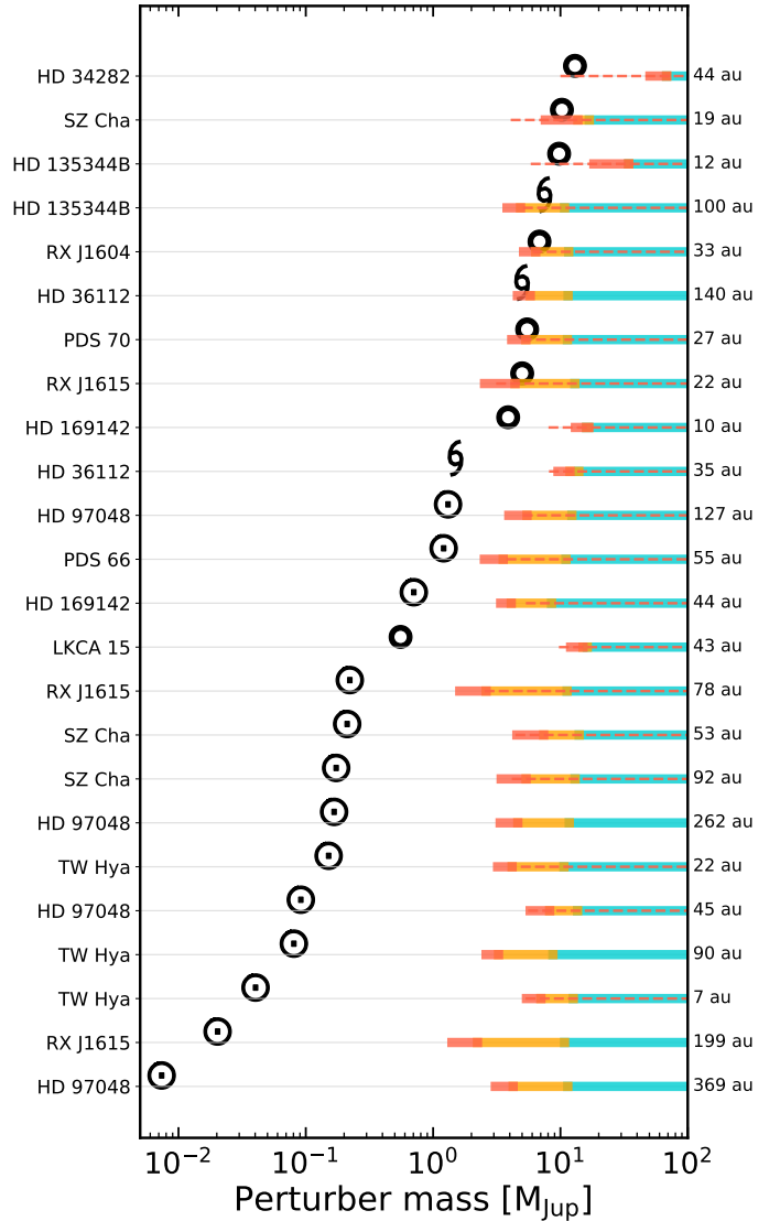
Fig. 7. Population of perturbors from Fig. 6 compared to our derived 5\sigma deprojected mass sensitivities at their location, which is shown on the right side of the figure. SPHERE/IRDIS with AMES-DUSTY, BEX-HOT, and BEX-WARM initial starts are shown as red, orange, and blue bars, respectively. The dashed lines correspond to SPHERE/IFS-ASDI contrasts and AMES-DUSTY post-formation luminosity.
