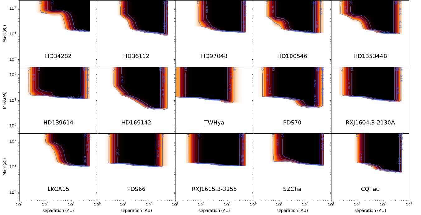
Fig. C.3. Same as C.1, but for BEX-WARM conditions.
