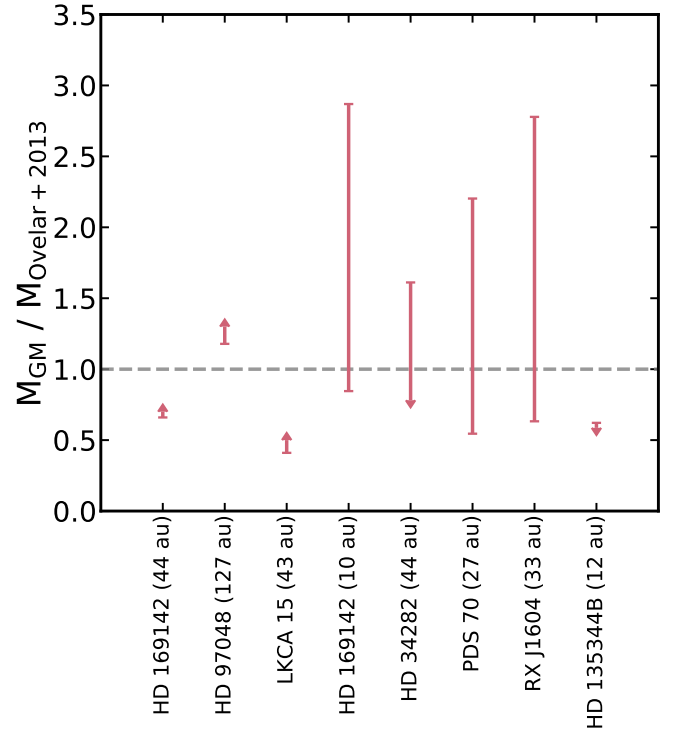
Fig. 10. Difference in the estimated mass of the perturbors of Fig. 6 ( M_{GM} ), calculated using the gap morphological features observed only in scattered light, and those calculated via de Juan Ovelar et al. (2013), which compares the cavity sizes in scattered light and the millimetre continuum ( M_{Ovelar+2013} ). The only assumed uncertainties are those linked to the location of the scattered-light inner edge of Eq. (5).
