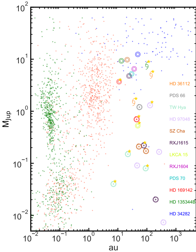
Fig. 6. Underlying population of potential perturbors derived from PPD substructures in the SPHERE scattered-light images. For planets in the gaps between rings (circles with inner dots) and planets in cavities (circles), these values are estimated using a proportionality factor of 8 R_{\text{Hill}} to account for the mass that would create the observed width in the scattered-light gap (Eq. (1)). When the gap morphology in scattered light was taken into account, planet masses are taken from detailed simulations in the literature for \alpha = 10^{-3} , and are marked with an asterisk. Simulated planets creating spiral features are also included as spiral symbols (see references in the Appendix A and see also Fig. A.1). The distributions of confirmed planets in the exoplanets.eu catalogue are shown as small dots: green (radial velocity discoveries), orange (transits), and blue (imaging).
