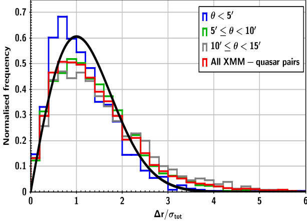
Fig. 5. Distribution of position-error-normalised offsets between 3XMM-DR5 X-ray sources and SDSS quasar counterparts (red histogram). The expected Rayleigh distribution is overlaid (black). The XMM position errors are as provided in the 3XMM catalogues (i.e. unadjusted, with no scaling or systematic included). Also shown are similar histograms for data from EPIC off-axis angles, \theta , in the ranges \theta < 5' (blue), 5' \leq \theta < 10' (green) and 10' \leq \theta < 15' (grey). The data are normalised to unit area.
