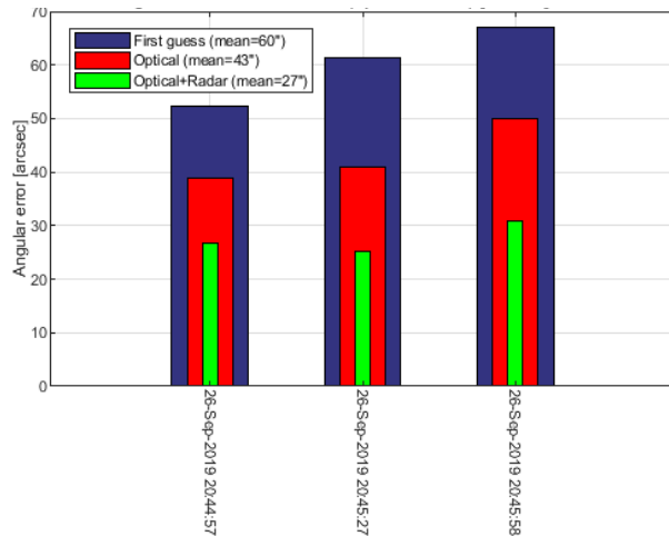
Figure 17: Results of the orbit determination for TLE improvement performed combining F-H (optical) and F-H-I (optical + radar) sets of measures. TLEs accuracies have been assessed by comparing the residuals with respect to measures of the N set.
