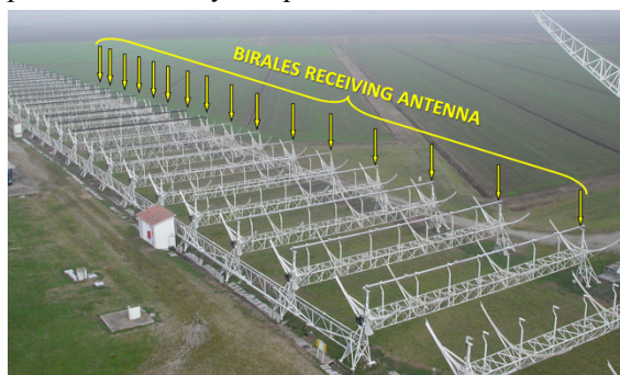
Figure 4: BIRALES receiving antenna
