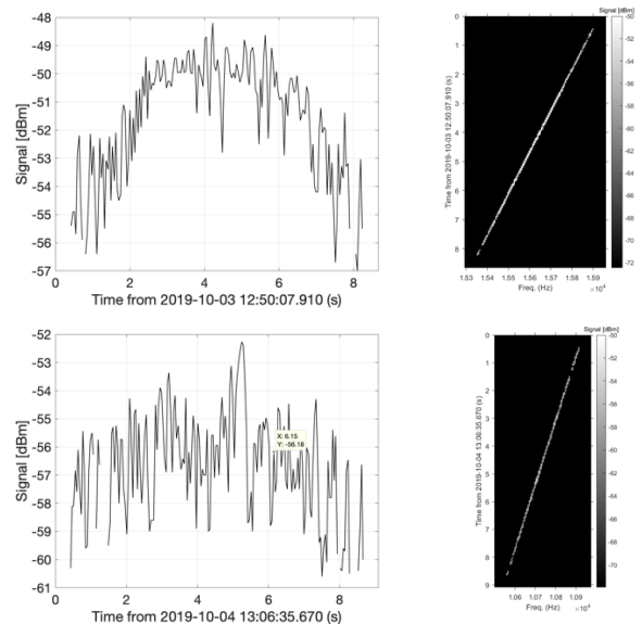
Figure 14: Signal received by BIRALES during two passages of Jason2.
