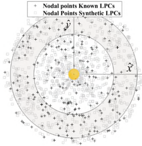
Figure 3. Nodal point distribution in the ecliptic plane for all known LPCs and Boe et al. synthetic population [5].
