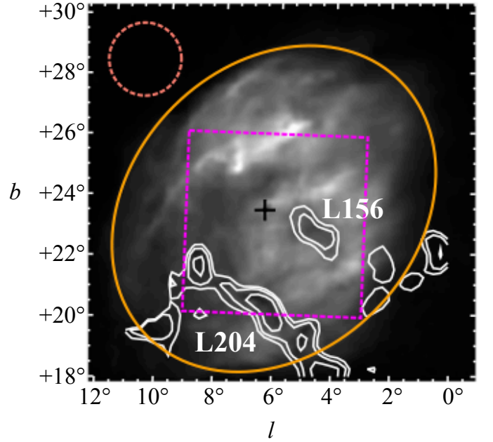
Fig. 1. Selected regions and the dark clouds (this work) overlaid on the I_{H\alpha} map of Sh 2–27. The dashed circle with a radius of 1''.2 is chosen to estimate the off-region used in RM_{\text{Sh2-27}} estimation (see Sect. 5.3). The dashed box is used for the SF calculations. Each side of the box is \sim 6'' . Contours from the CO emission map of Dame et al. (2001) are overlaid on the H II region to display the structure of the dark clouds. The plus sign represents the location of \zeta Oph at (l, b) = (6^\circ.3, +23^\circ.6) . The greyscale range is 0–2000 dR.
