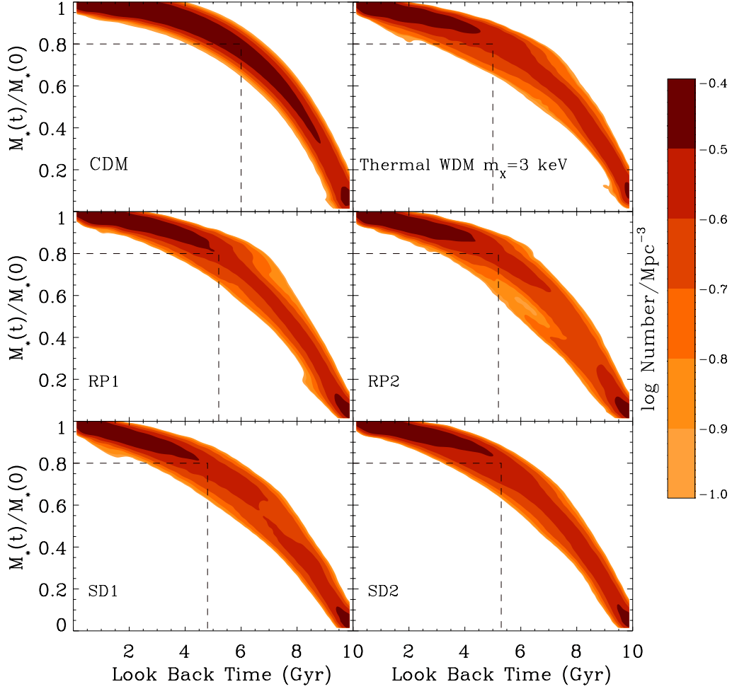
Figure 8. The predicted stellar growth histories for the DM models indicated by the labels. The contours show, at given look-back time, the number of model galaxies with a given ratio M_*(t)/M_*(0) between the mass formed in all progenitors of the final galaxies and the final stellar mass. Only galaxies with final mass 9 \leq \log M_*/M_\odot \leq 9.5 are considered. The dashed line show the look-back time corresponding to the formation of 80% of the final stellar mass.
