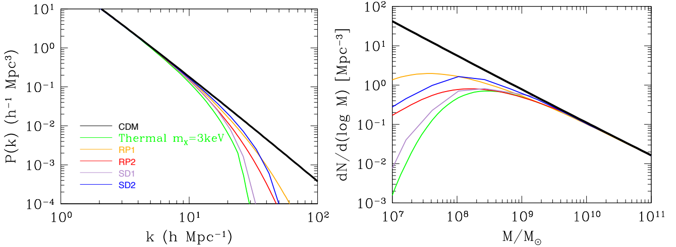
Figure 1. Left panel: The linear power spectrum at z=0 for the different DM models considered in the text, as indicated by the labels. Right panel: for the same DM models, we show the DM halo mass function at z=0 .
