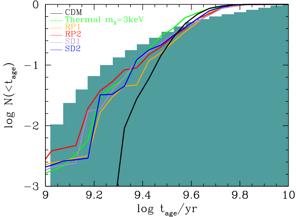
Figure 10. For the different DM scenarios considered in the text, we plot the predicted cumulative distributions of the mass-weighted age t_{age} for the different DM models (solid lines), and compare them with the data by Gallazzi et al. (2008, solid histogram) weighted as described in Calura, Menci, Gallazzi (2014; see text). In the plot we have considered all galaxies with M \geq 10^9 M_{\odot} .
