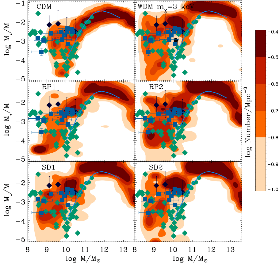
Figure 4. The stellar-to-halo mass ratio M_*/M as a function of the halo mass M of model galaxies are shown as coloured contours for the different assumed DM models. These are compared with different sets of data from Ferrero et al. (2012, black points), Brook and Di Cintio (2015, green points) and Read et al. (2017, blue squares). For the latter we excluded the Leo T data where no rotation curves are available. The blue line is the average relation obtained for CDM by Guo et al. (2011) using a semi-analytic model applied to large cosmological N-body simulations.
