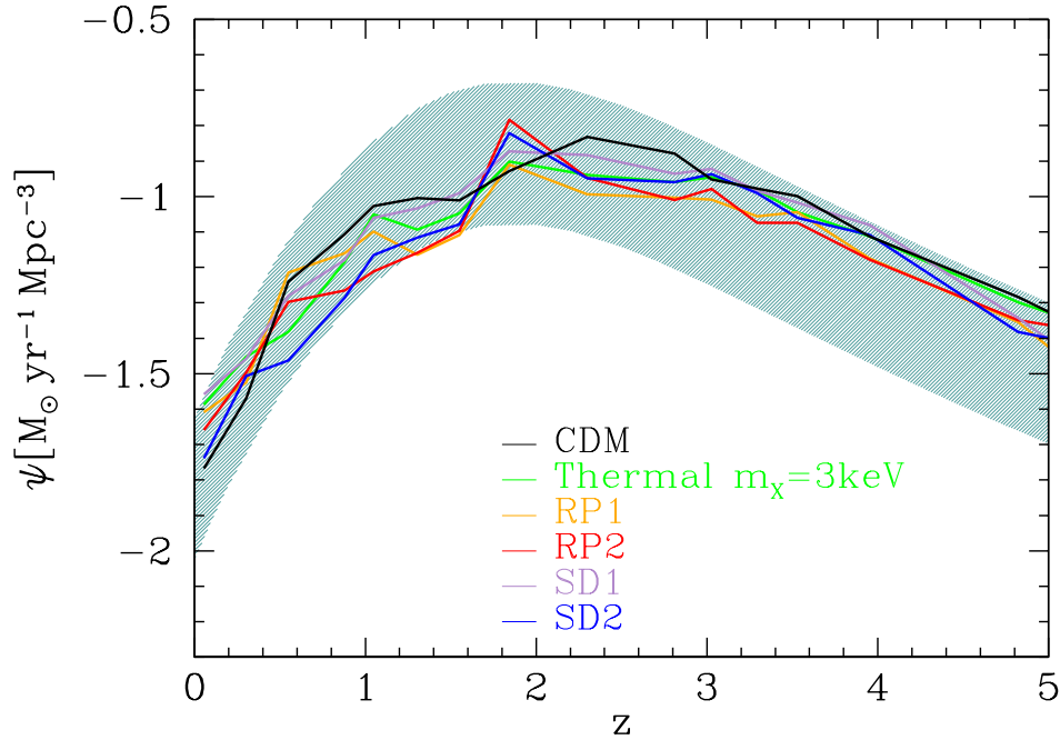
Figure 7. We show the predicted star formation rate density for the different DM models considered in the text and shown by the labels. The shaded region corresponds to the present uncertainties as result from the compilation of data in Madau & Dickinson (2014), who consider only surveys that have measured SFRs from rest-frame FUV (generally 1500Å), MIR, or FIR measurements, and including all galaxies with luminosities larger than 0.03 L_* , where L_* is the characteristic luminosity of the considered data sample. For the model predictions, we adopted the same lower luminosity cut, deriving L_* as the ratio between the second and the first moment of the UV luminosity functions.
