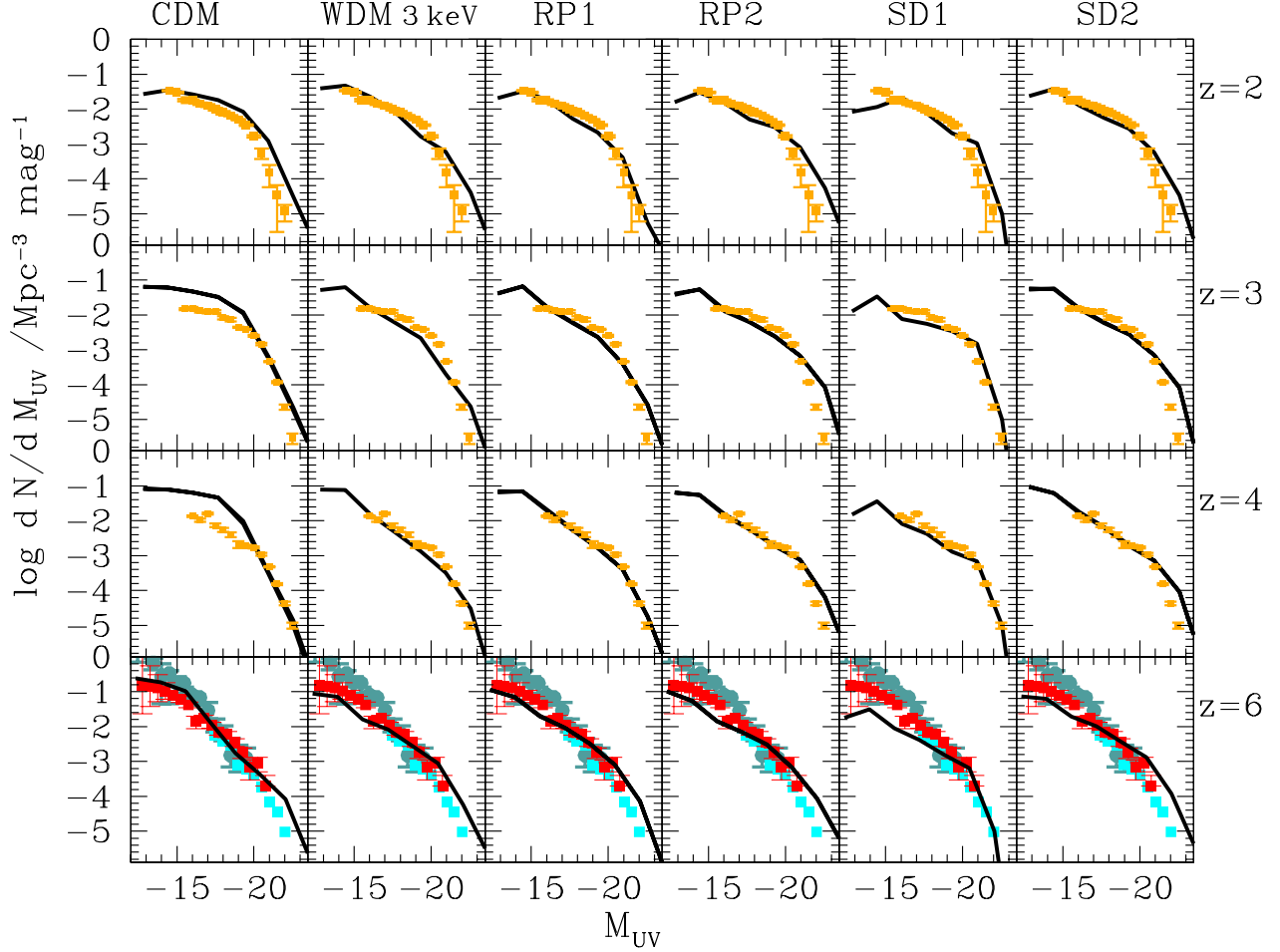
Figure 6. The evolution of the predicted UV luminosity function for the different DM models considered in the text and indicated at the top of the plot is shown for the different redshifts indicated on the right. Data for z \leq 4 are taken from Parsa et al. (2016). Data in the highest redshift bin are taken from Livermore, Finkelstein & Lotz (2017, dark green circles), from Bouwens et al. (2017a; red squares) for the faint end, while for the bright end we compare with Finkelstein et al. (2015a, light cyan squares).
