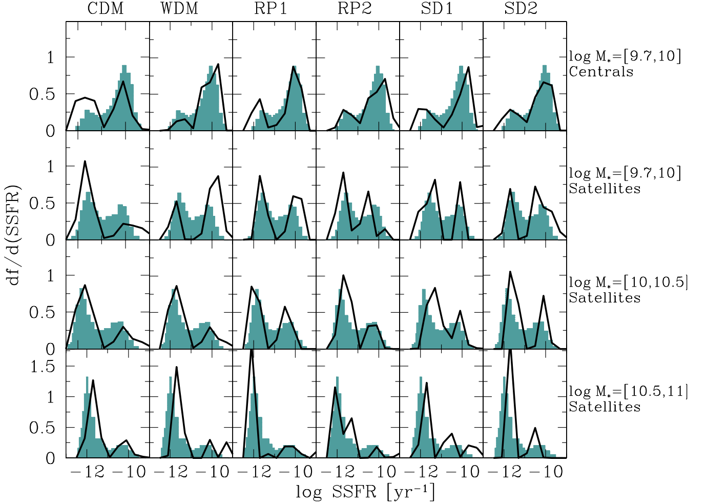
Figure 9. Predicted distributions of specific star formation rate (solid lines) for central and satellite galaxies in different mass bins as indicated by the labels, for the different DM models indicated on the top. The solid histograms are the observed distributions measured by Wetzel et al. (2013).
