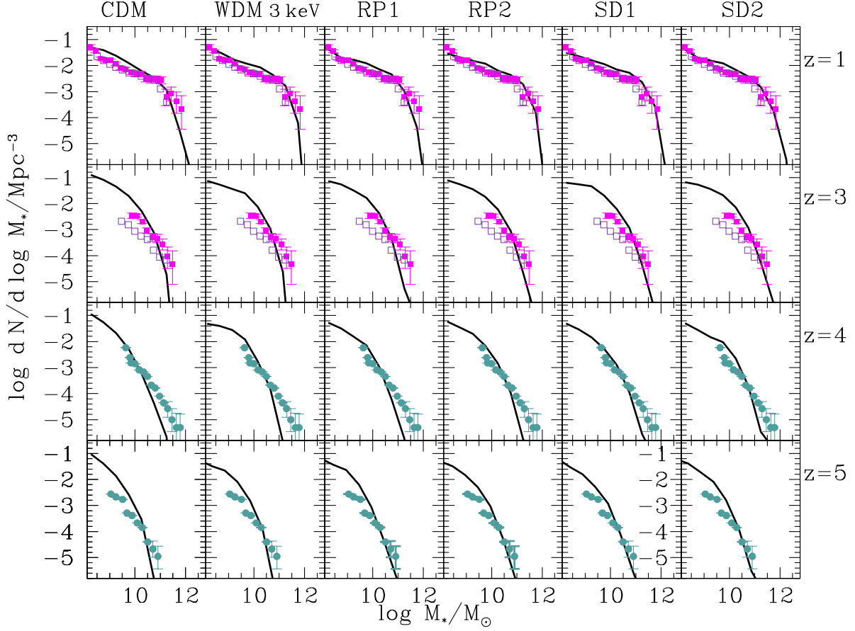
Figure 5. The evolution of the predicted stellar mass function for the different DM models considered in the text and indicated at the top of the plot is shown for the different redshifts indicated on the right. Data for z \leq 3 are taken from Santini et al. (2012, filled squares) and Tomczak et al. (2014, open squares), while for z \geq 4 are taken from Grazian et al. (2015).
