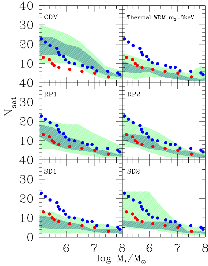
Figure 3. The stellar mass function of satellites of Milky Way-like galaxies in the models are represented as shaded regions enclosing 68 % (darker) and 95 % (lighter) of the satellites of halos with DM mass in the range M = 1 - 2.5 \cdot 10^{12} M_\odot . These are compared with the compilation of observational data by McConnachie (2012) for the Milky Way satellites (red dots) and for the satellites of M31 (blue dots).
