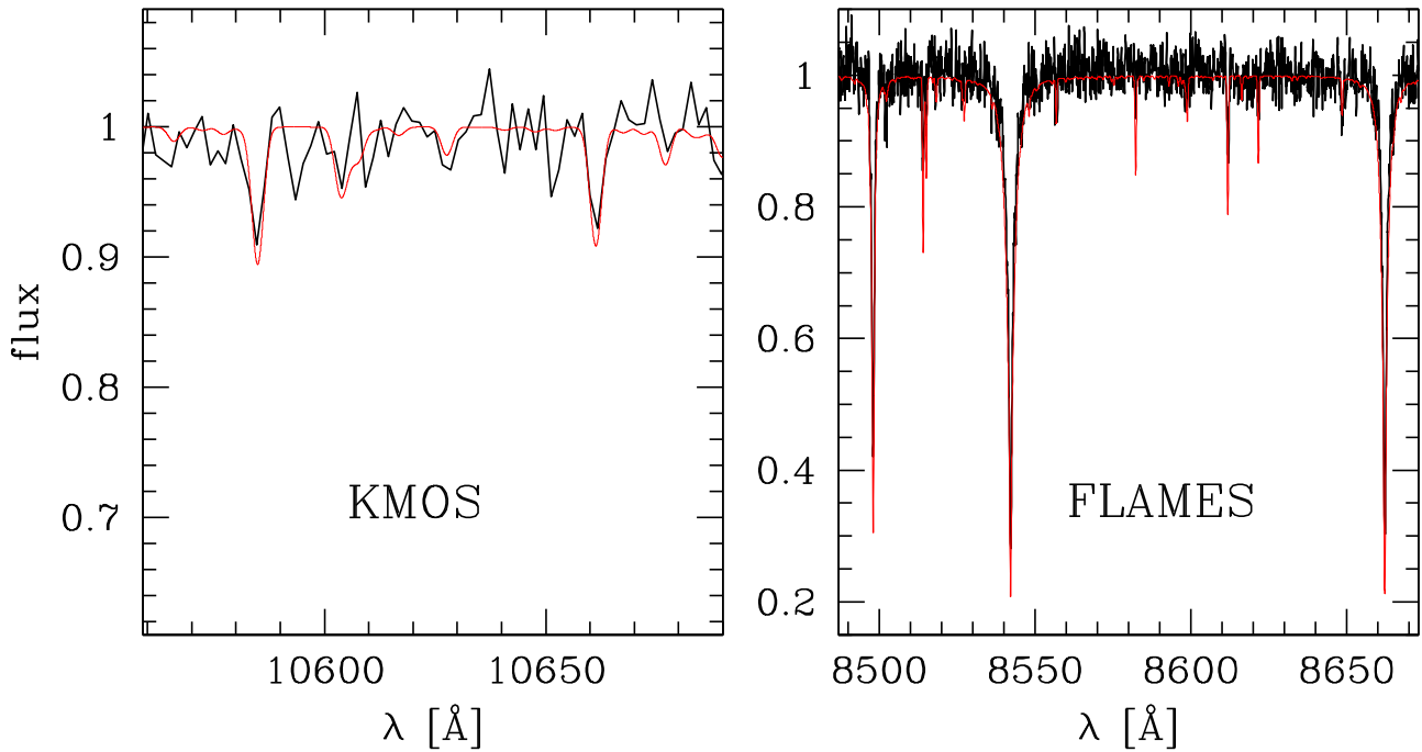
Figure 1. Examples of KMOS (left) and FLAMES (right) spectra. The observations are plotted in black, while the synthetic templates are in red. Fluxes are arbitrarily normalized to unit.
