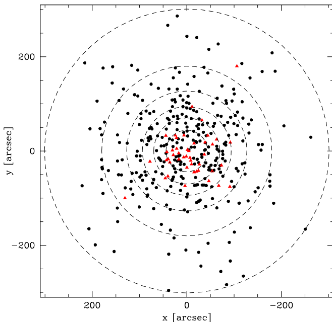
Figure 4. Position the surveyed kinematic members in the plane of the sky. Symbols have the same meaning as in Figure 3. The plotted coordinates, x and y , are the R.A. and decl. relative to the cluster center, determined by using Equation (1) in van de Ven et al. (2006). The dashed circles mark the boundaries of the radial bins used to determine the cluster velocity dispersion (see Table 3).
