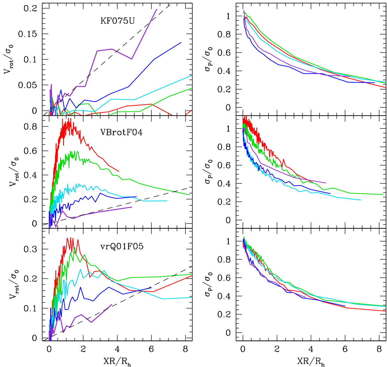
Figure 8. Time evolution of the rotation curve (left-hand panels) and velocity dispersion profile (right-hand panels), both calculated from line-of-sight velocities and normalized to the central velocity dispersion, for three of the N -body simulations from Tionco et al. (2016a). The radius is normalized to the projected half-mass radius, R_h . Different lines correspond to different dynamical stages, with the red, green, cyan, blue, and purple lines corresponding to increasing dynamical ages. In the left panels, a dashed line shows a theoretical solid-body rotation curve with slope \Omega/2 , a value that star clusters will converge to during their long-term evolution in a tidal field (see Tionco et al. 2016b). In all cases, both sets of kinematic profiles have been calculated by considering all stars enclosed within one Jacobi radius.
