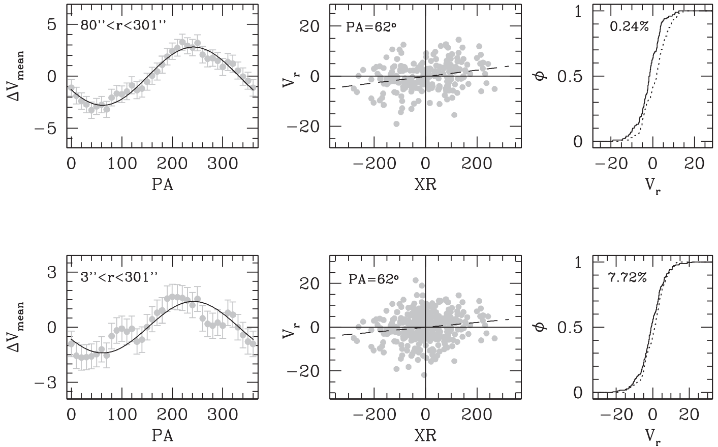
Figure 5. Diagnostic diagrams (see Section 3.2) of the rotation signatures detected at r > 80'' (upper row) and over the entire radial range surveyed (lower row). Left panels: difference between the mean line-of-sight velocity calculated in the two half-planes, as a function of the position angle of the dividing line. The labels indicate the radial range considered. Central panels: spatial distribution of the radial velocities (in \text{km s}^{-1} ). XR denotes the projected distance from the best-fit rotation axis (in arcsec), with the value of the position angle marked. Right panels: cumulative distribution of the RVs with positive (dotted line) and negative (solid line) projected distance XR . The outcome of a KS test of the two distributions is reported in the top left corner of each panel.
