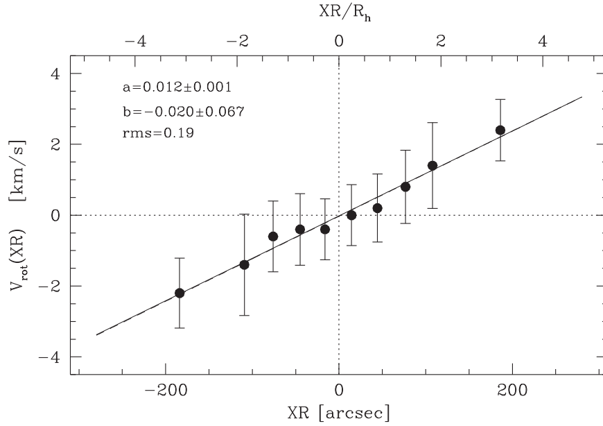
Figure 6. Rotation curve of NGC 5986. The mean velocity as a function of the distance from the rotation axis is displayed (see also Table 2). The best-fit line to the observed behavior has slope ( a ), intercept ( b ), and rms scatter ( \text{rms} ) as labeled in the figure.
