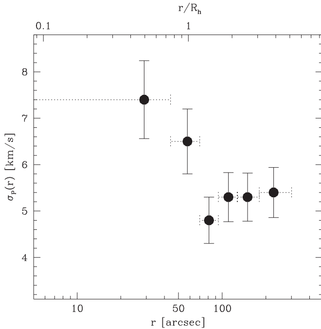
Figure 7. Projected velocity dispersion profile, determined after subtraction of the rotational contribution to the individual RVs, in six concentric annuli around the cluster center.
