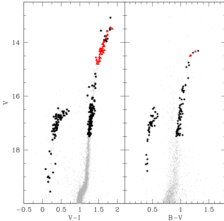
Figure 3. Position of the surveyed kinematic members in the color–magnitude diagrams of NGC 5986. The KMOS targets are highlighted as red triangles, while the stars surveyed with FLAMES are plotted as black circles.
