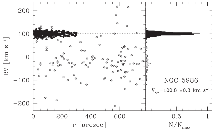
Figure 2. Left panel: radial distribution of the line-of-sight velocities measured from the MikiS observations in NGC 5986. The selected cluster members are plotted as black circles, while field contaminants are in gray. Right panel: RV distribution as a normalized histogram. V_{\text{sys}} denotes the cluster systemic velocity.
