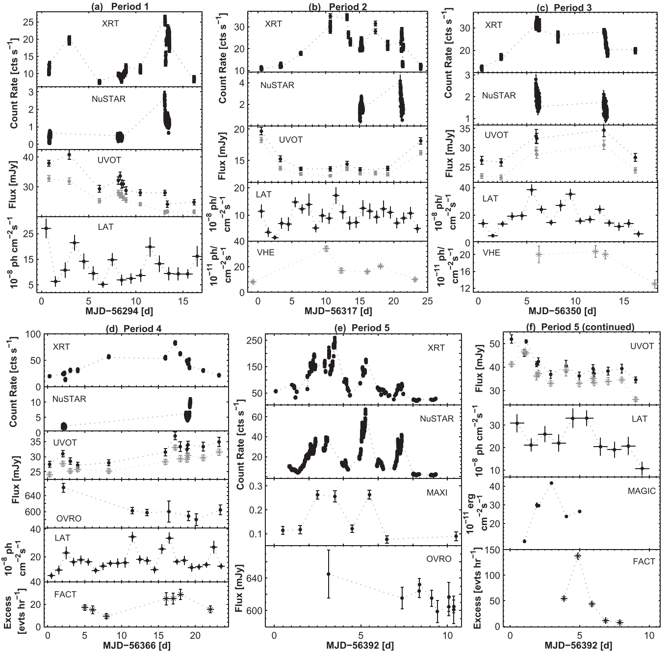
Figure 2. MWL variability of Mrk 421 in different epochs. In each UVOT panel, the UVW1 -band light curve is plotted with black points, and a gray color is used for the UVW2 band.
