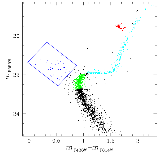
Figure 4. Decontaminated CMD of NGC 339. In blue, we selected BSSs, and in red, green, and cyan, the stars belonging to the RC, TO, and RGB regions, respectively.
