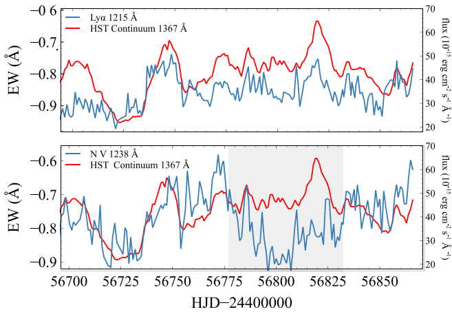
Figure 2. Both panels show the arbitrarily scaled FUV continuum in red, as a function of Heliocentric Julian Date -24,400,000 . The upper panel shows the equivalent width of the Ly \alpha absorber of Component 1 in blue and the lower panel shows the equivalent width of the corresponding N V \lambda 1238 absorption line. Shaded area indicates the time in which the “holiday” is happening.
