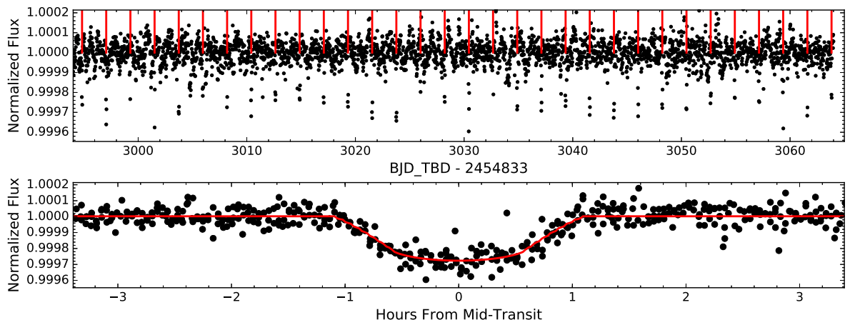
Figure 1. Top: normalized flux of K2 light curve with red tick-marks indicating the transit times. Bottom: phase-folded transit data (black points) including our model fit (red line).
