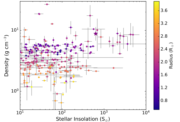
Figure 8. Density vs. stellar insolation for planets with radii smaller than 4\text{ }R_{\oplus} . Point color indicates the radius of the planet. K2-291 b (star) exhibits a density similar to other small, close-in planets.
