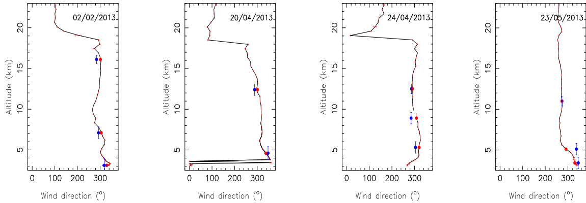
Figure 9. Examples of WD estimates as measured by GeMS (blue dots) and retrieved by Meso-NH (vertical profile – black continuous line) during different nights. Error bars with respect to the y-axis are the same as those of the wind speed case. Error bars along the abscissa are of the order of a few degrees and therefore not visible in the picture. The selected nights are the same as those related to Fig. 6. Typically GeMS identifies no more than three layers for the WS. The red dots are displayed on the vertical profile simply to indicate the same heights as the blue dots and facilitate the comparison. [A colour version of this figure is available in the online version.]
