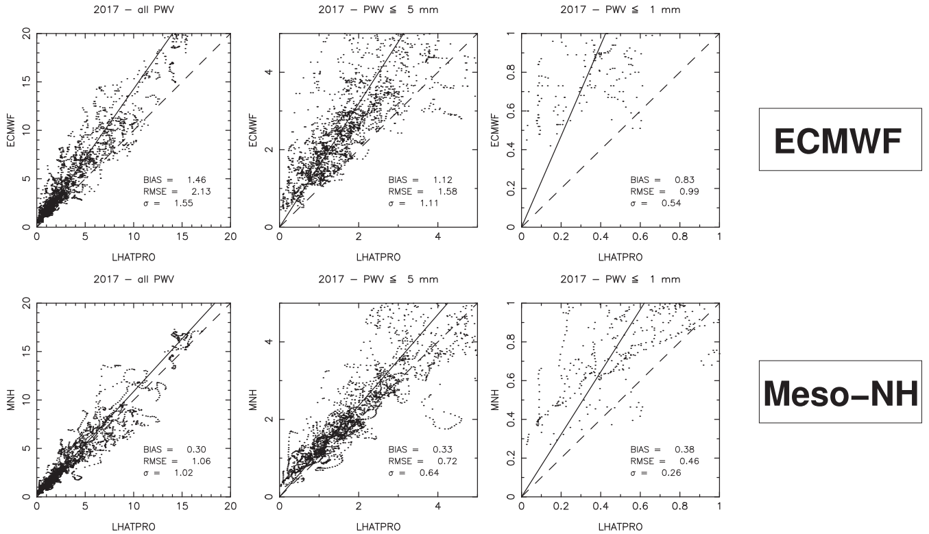
Figure 4. Cerro Paranal – scatterplot computed on the 135 nights 2017 sample comparing LHatPRO measurements either with ECMWF GCM forecasts ( top row ) and MNH forecasts ( bottom row ). The plots are relative to the whole sample (first column), to a sample filtered by selecting LHatPRO measurements with PWV \leq 5 mm (second column) and PWV \leq 1 mm (third column). The dashed line corresponds to the 45^\circ that should represent a perfect match between model and measurements. The straight line corresponds to the regression line computed on the data points.
