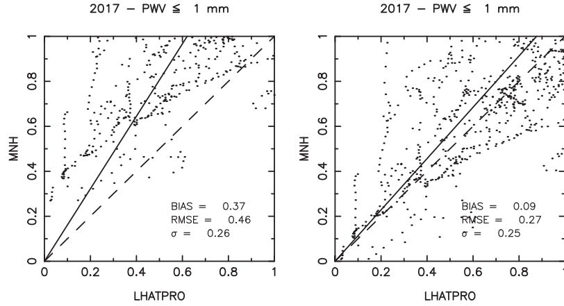
Figure 3. Cerro Paranal – scatterplot computed on PWV. The plots are computed over the 35 nights 2017 sample obtained by selecting all nights on 2017 with PWV \leq 1 mm for, at least, 30 per cent of the night. In the left-hand panel, we show the uncorrected (raw) scatterplot, while in the right-hand panel we show the scatterplot obtained with correction in equation (6). The indicators are computed by filtering the sample selecting LHATPRO measurements with PWV \leq 1 mm. The dashed line corresponds to the 45^\circ that should represent a perfect match between model and measurements. The straight line corresponds to the regression line computed on the data points.
