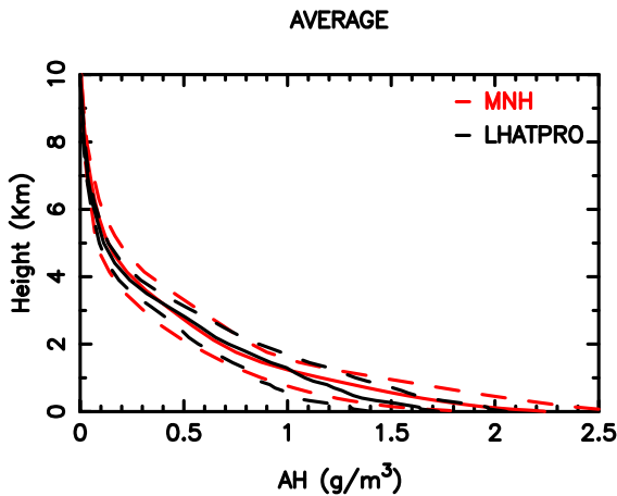
Figure 5. Cerro Paranal – average vertical AH profiles computed over the 120 nights 2013 sample by the MNH model (red) and by LHatPRO (black line). Dash lines indicate the standard deviation for the model (red) and LHatPRO (black).
