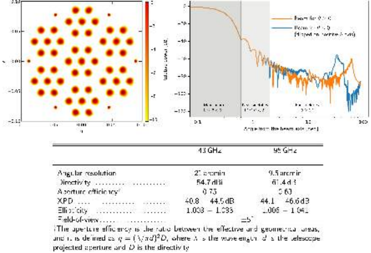
Figure 5. Left: footprint of the LSPE-Strip main beams in the (u, v) plane (large beams, 43 GHz, small beams, 95 GHz). Right: beam cut for \phi = 0 of the central horn. We have flipped the beam section for \theta < 0 on the positive axis to better highlight the asymmetries. The (u, v) variables are defined as u = \sin(\theta) \cos(\phi) , v = \sin(\theta) \sin(\phi) , where (\theta, \phi) are standard spherical coordinates, with the center of the telescope pointing towards \theta = 0 . The inset table reports the averaged main optical parameters.
