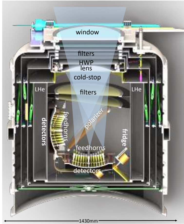
Figure 13. LSPE-SWIPE cryostat and optical system. Radiation enters from the top window, passes across filters, HWP, lens, cold-stop, and other filters. It then is split by the large wire grid and collected in the two curved focal planes.
