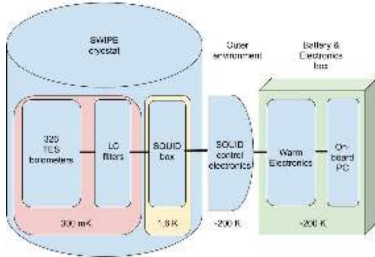
Figure 18. Schematic of the LSPE-SWIPE readout with the indication of the temperatures of the different stages.
