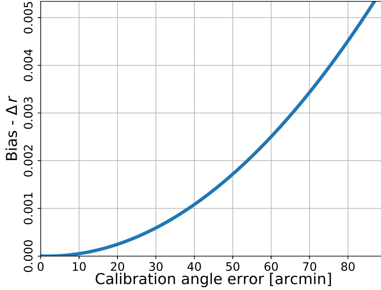
Figure 20. Bias in r due to a rotation in the polarization angles. The bias is computed by adding a rotation to the polarization angles, and estimating the tensor-to-scalar ratio r from pixel based likelihood as described in section 5.2.
