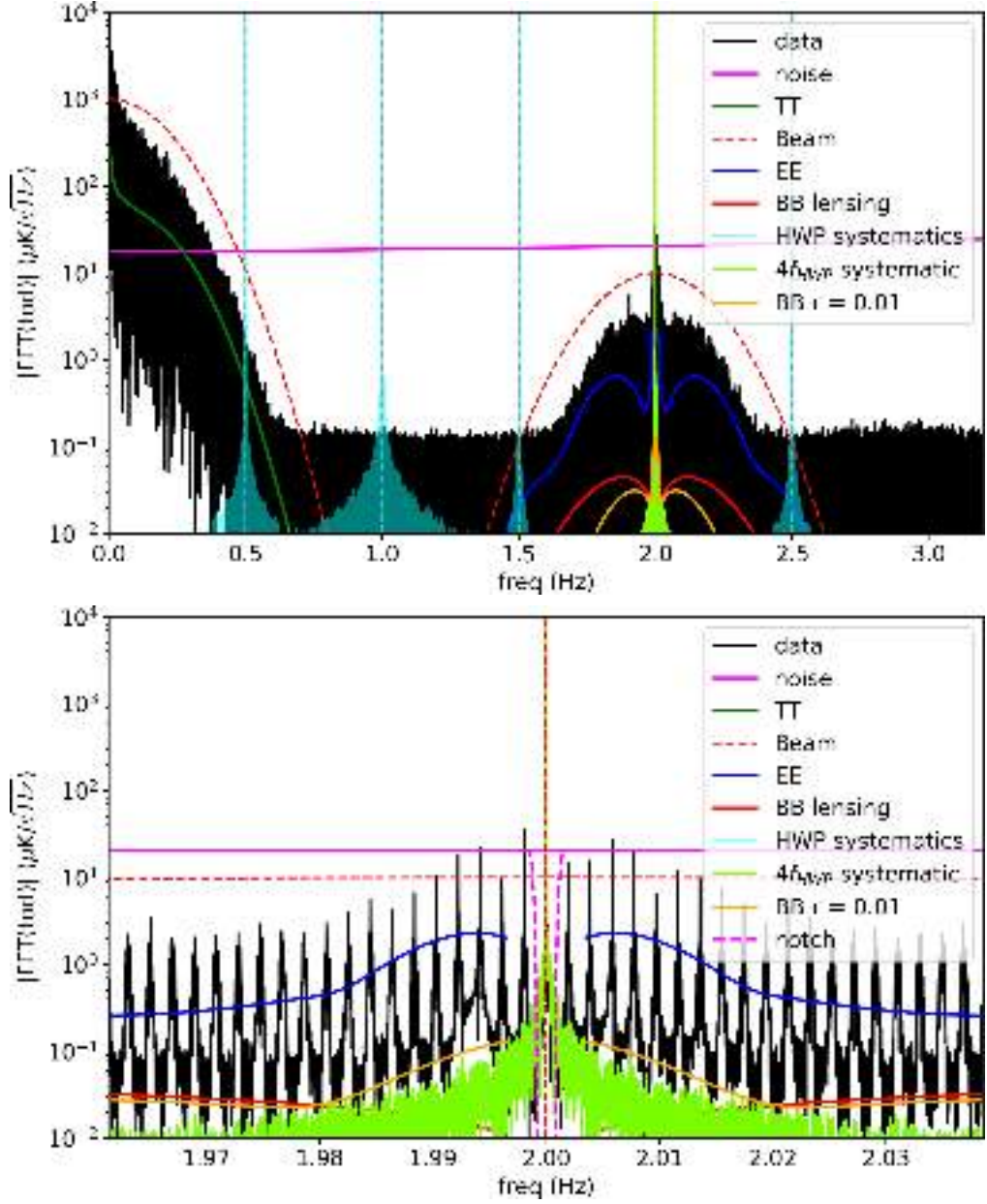
Figure 21. LSPE-SWIPE frequency spectrum ( top ), and zoom-in near modulation frequency ( bottom ), for a 16 hours noise-free CMB-only simulated timestream. The black curve represents the data; CMB temperature data are centered around 0 frequency, and polarization data around 4f_{\text{HWP}} . The magenta line is the noise for a single detector at 145 GHz. The magenta dashed line, is the noise multiplied by the notch filter. Vertical dashed lines represent harmonics of the HWP spin frequency. The dark green curve is the expected signal for a temperature CMB angular power spectrum, blue curve for E-mode power spectrum, red for B-mode (lensing only) and orange for inflationary B-mode. The light-green curve, visible in the bottom plot, is a systematic effect at 4f_{\text{HWP}} , with an amplitude of 1 mK, spread in frequency due to the uncertainty in the HWP angular velocity \sigma_{\omega_{\text{HWP}}}/\omega_{\text{HWP}} = 0.6 \times 10^{-6} . The cyan clear curves are the systematic effects at 1, 2, 3, 5f_{\text{HWP}} , as discussed in section 4.3.3. Since the signal is quasi-periodic, with period T_{\text{payload}} , its Fourier transform peaks at the modulation frequency 4f_{\text{HWP}} and then in frequency shifts equal to \Delta f = 1/T_{\text{payload}} , clearly visible in the bottom figure.
