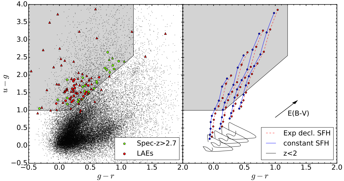
FIG. 3.— Left: u-g vs g-r colors of all r -band detected sources are shown in dots together with the LBG selection indicated by a grey shaded region. Red symbols are photometric LAEs while green symbols are known spectroscopic sources at z_{\text{spec}} \geq 2.7 . All sources that are not detected in the u -band are shown as triangles using the 2\sigma limiting magnitude. Right: the redshift evolution of colors are illustrated for galaxies with dust reddening values. E(B-V)=0, 0.1, 0.2, 0.3 (from left to right). Galaxy's star formation rate is modeled to be constant (blue) or declining exponentially with time (red) as \psi \propto \exp(-(t/100 \text{ Myr})) . Along a given track, source redshift increases from z = 2.7 upwards with the interval \Delta z = 0.1 . Black lines show expected colors of local spiral galaxies when redshifted out to z = 2 .
