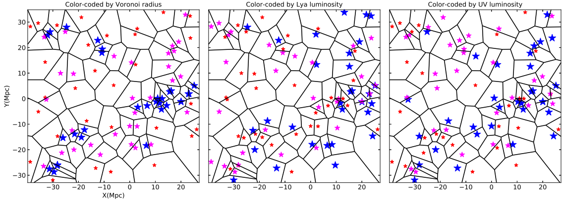
FIG. 8.— Voronoi tessellated maps of the LAE positions. The LAE sample is divided by Voronoi radius (left), \text{Ly}\alpha luminosity (middle), and UV luminosity (right) of each LAE. In all panels, blue, pink and red colors are used for the top, middle, and bottom third, corresponding to r_V \leq 3.2 , 3.2 < r_V \leq 4.85 , and r_V > 4.85 in Voronoi radius, \log(L_{\text{Ly}\alpha}) > 42.60 , 42.38 < \log(L_{\text{Ly}\alpha}) \leq 42.60 , and \log(L_{\text{Ly}\alpha}) \leq 42.38 in line luminosity, and \log(L_{\text{UV}}) > 28.06 , 27.68 < \log(L_{\text{UV}}) \leq 28.06 , and \log(L_{\text{UV}}) \leq 27.68 in UV luminosity. The correlation between these parameters is evident as a large fraction of UV-/Ly \alpha -luminous galaxies are found in the LAE overdensity region.
