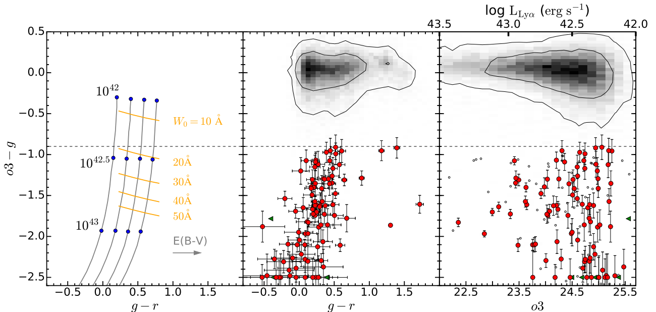
FIG. 2.— Left : Theoretical tracks for LAEs of different luminosities and dust reddening in the o3 - g vs g - r color diagram. The grey lines show the color evolution with increasing \text{Ly}\alpha luminosities (from top to bottom) at four reddening values ( E(B - V) = 0 - 0.3 in steps of 0.1 from left to right). Blue points show the \text{Ly}\alpha luminosities, 10^{42.0} , 10^{42.5} and 10^{43.0} \text{erg s}^{-1} at the continuum g band magnitude of 25.5. Orange lines represent the \text{Ly}\alpha rest-frame equivalent widths ( W_0 ) of 10, 20, 30, 40, and 50 Å. The o3 - g color cut (dashed horizontal line) approximately corresponds to W_0 \gtrsim 20 Å. Middle : the color-color diagram for all o3 detected sources. The two contour lines enclose 68% and 95% of the sources. Galaxies that satisfy the LAE criteria are indicated as red circles; those undetected in g or r band are shown as green triangles. Galaxies with o3 - g \leq -2.5 are shown at the color position of -2.5 . Right : o3 - g color as a function of o3 -band magnitude. Sources that do not meet the u - g color cut are shown in open circles. The approximate \text{Ly}\alpha luminosities corresponding to the o3 magnitude are indicated on the upper abscissa.
