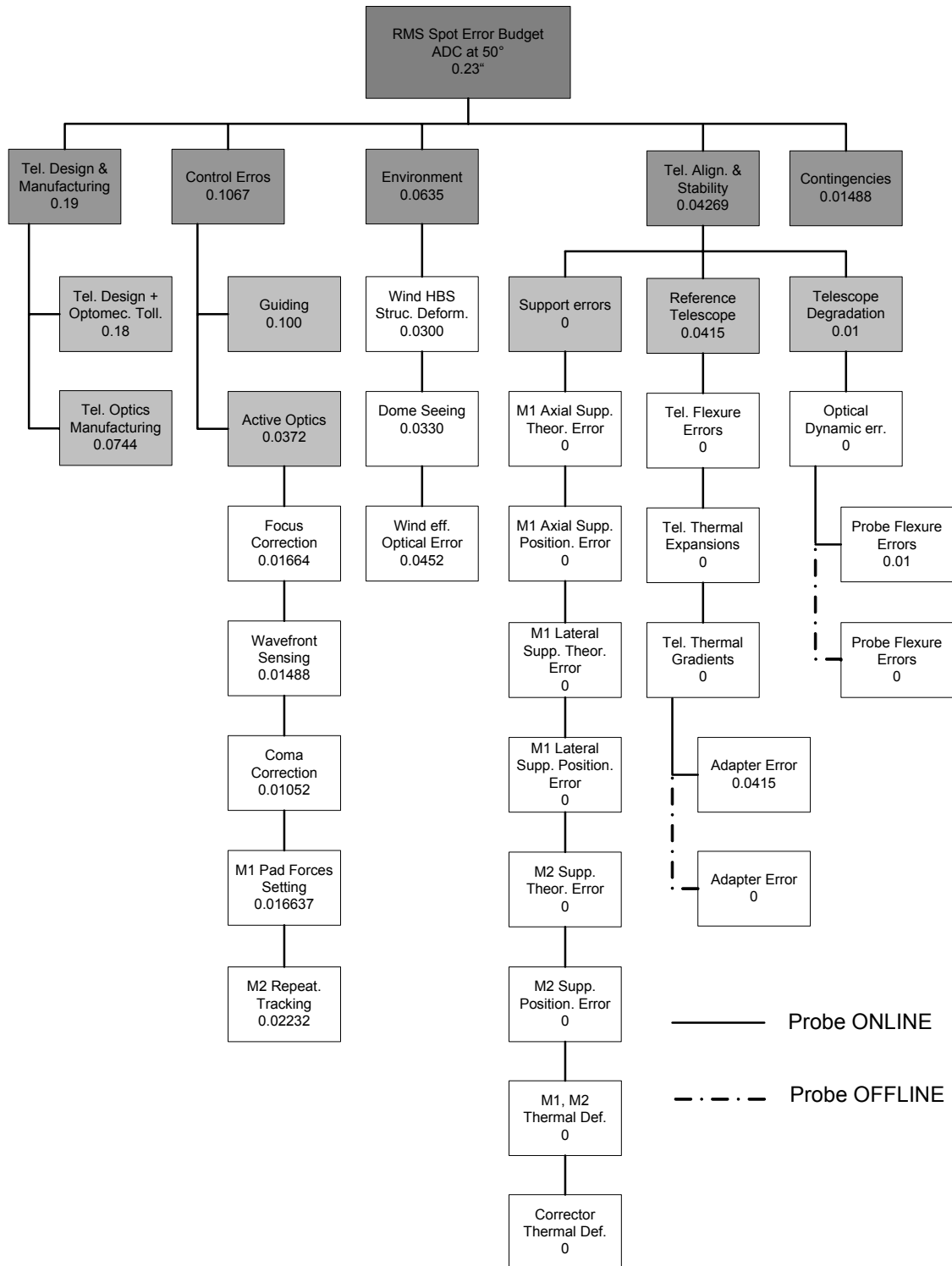
Figure 5: VST Image Quality budget in terms of RMS spot radius, for ADC corrector configuration at 50^\circ zenith angle
