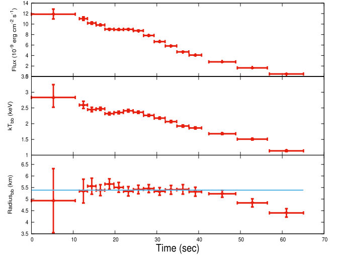
Figure 9. Evolution of the 0.3–10.0 keV flux (top panel), the blackbody temperature (centre panel) and emission radius (bottom panel) obtained by flux-bin spectra obtained by stacking all of the type-I bursts. Beyond 40/50 s after the peak the statistics of the single spectra is very low and the spectral parameters are not reliable. The emission radius, modified by the colour correction factor ( 1.35 \pm 0.05 ), is consistent with a NS radius of 6.97–7.6 km.
