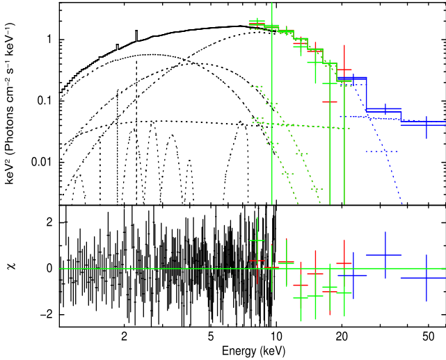
Figure 5. Unfolded E^2 f(E) XMM-Newton/EPIC-pn (black), INTEGRAL/JEMX-1 (red) and JEMX-2 (green) and INTEGRAL/ISGRI (blue). The dashed curves represent the best-fitting continuum (DISKBB, BB, NTHCOMP and POWER-LAW components) plus nine additional narrow and broad emission lines (see text).
