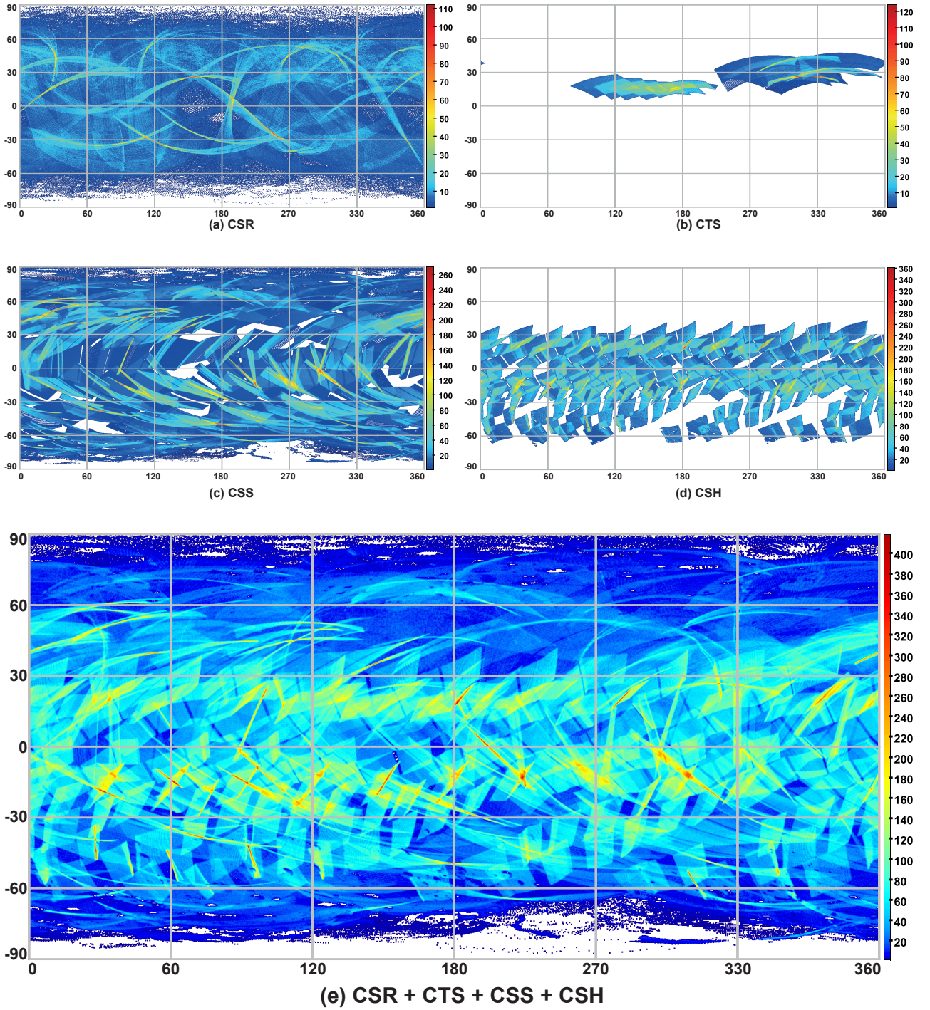
Fig. A.1. Density maps of the VIR visible data set used in the study. Panel A: CSR mission phase; panel B: CTS; panel C: CSS; panel D: CSH; and panel E: regroups every four. For details about the mission phases, see Table 1 and Sect. 2.2. Each map is built with TOPCAT with a Plate Carée projection (see Sect. 2.4), and observations are represented as points. The scale corresponds to the square root of the observation density.
