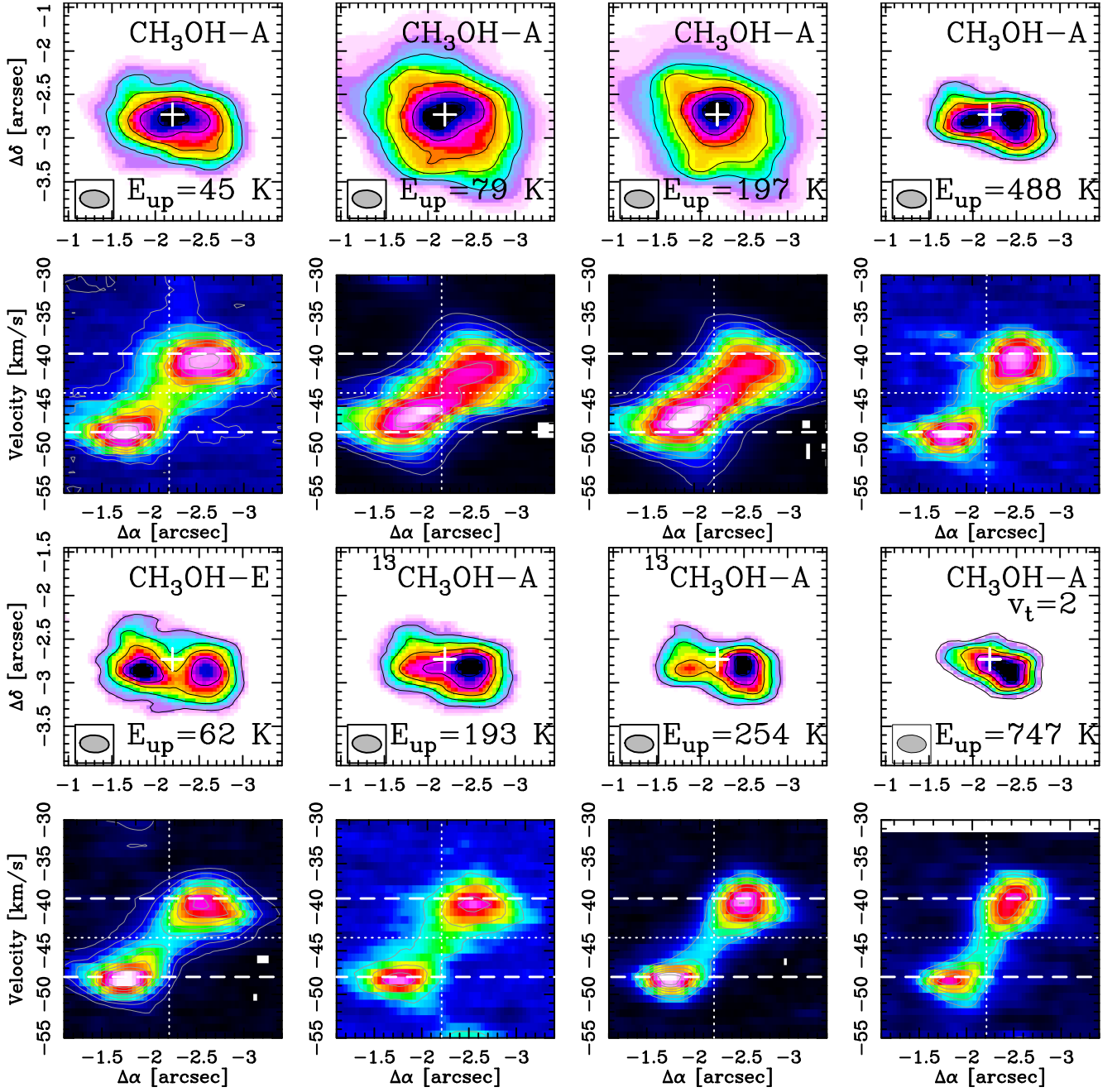
Fig. 5. CH 3 OH zeroth-moment map and pv -diagrams for the transitions listed in Table 1. The top row shows the zeroth-moment map calculated over a velocity range of [-55, -30] km s -1 ; contours start at 30% of the peak and increase by 15%. The white cross marks the position of the continuum peak. The beam is shown in the lower left corner. The symmetry of the methanol molecule is labelled in each panel, as well as the upper level energy of the transition. The subsequent row shows the pv -diagram along the \Delta\alpha axis and averaged over the extent of the cube, corresponding to \sim 2.5'' . The right-ascension offset of the continuum peak and the v_{\text{lsr}} velocity of the source are marked with a white dotted line. Dashed lines show v_{\text{lsr}} \pm 4.5 km s -1 , corresponding to the peak velocity of the CH 3 OH spots.
