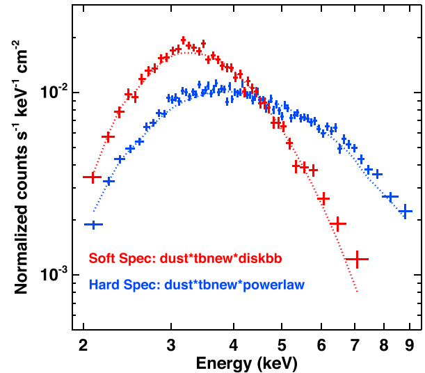
Figure 9. Combined, background-subtracted, Swift XRT spectra of the soft-state (red) and hard-state (blue) periods. The combined soft-state spectrum is well fitted by an absorbed disc blackbody ( N_H = 16.8 \times 10^{22} \text{ cm}^{-2} , kT_{\text{in}} = 0.80 \text{ keV} ), while the hard state by an absorbed power-law component ( N_H = 17.2 \times 10^{22} \text{ cm}^{-2} , \Gamma = 2.56 ).
