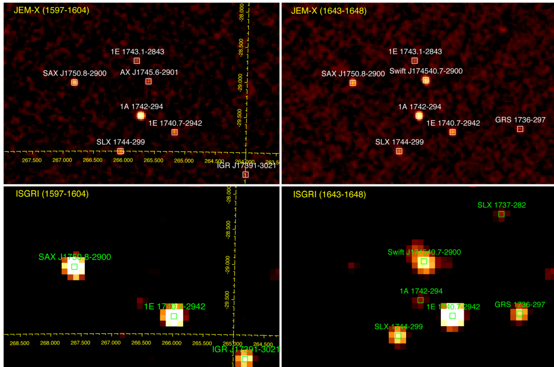
Figure 2. Mosaicked JEM-X (3–10 keV) and IBIS/ISGRI (20–40 keV) images around the position of Swift J174540.7–290015 obtained from the revolutions 1597–1604 performed before the source outburst (top and bottom left) and the revolutions 1643–1648 performed during the first part of the source outburst (top and bottom right). As it can be seen, Swift J174540.7–290015 is only detected from revolution 1643 onward in IBIS/ISGRI, while in JEM-X AX J1745.6–2901 is detected in the earlier revolutions at a position consistent with Swift (albeit at a much lower luminosity; see the text for details).
