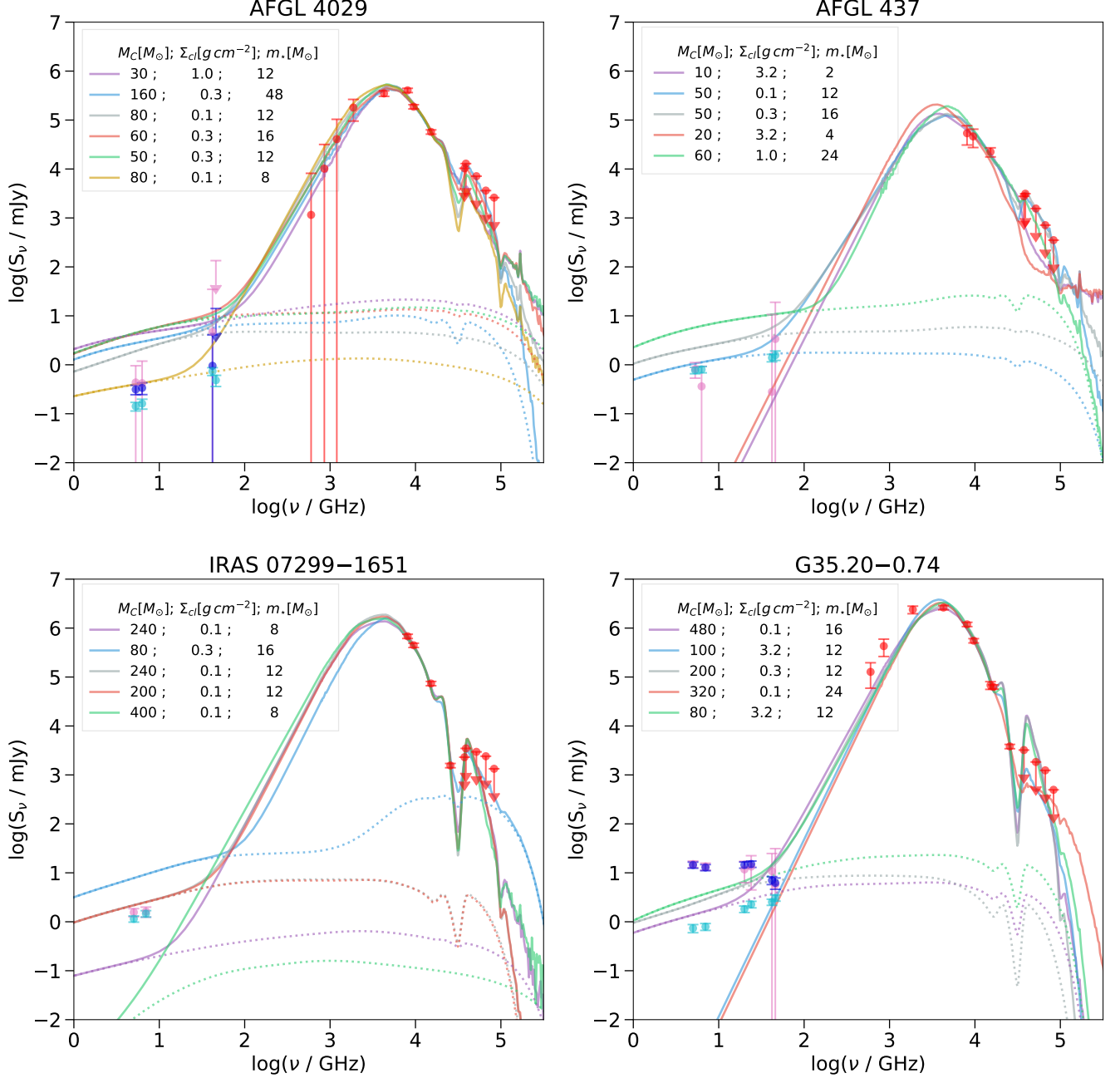
Figure 3. Comprehensive SEDs and models of the protostars. Red circles show IR data for the SOMA apertures as measured by DLT17. Solid colored lines are best fits to the IR data (except for yellow lines) from the ZT18 models, which have been augmented by including free-free emission from the TTZ16 model. The dotted colored lines correspond to the estimated free-free component using TTZ16, which only exceeds the thermal dust component at long wavelengths. For sources AFGL 4029 and IRAS 20126+4104 the yellow solid and dotted lines correspond to the best new model estimate of the total emission and the free-free emission, respectively. The colored circles correspond to the flux density as a function of frequency for each scale (magenta: SOMA; blue: Intermediate; cyan: Inner). Error bars are explained in §4.2.
