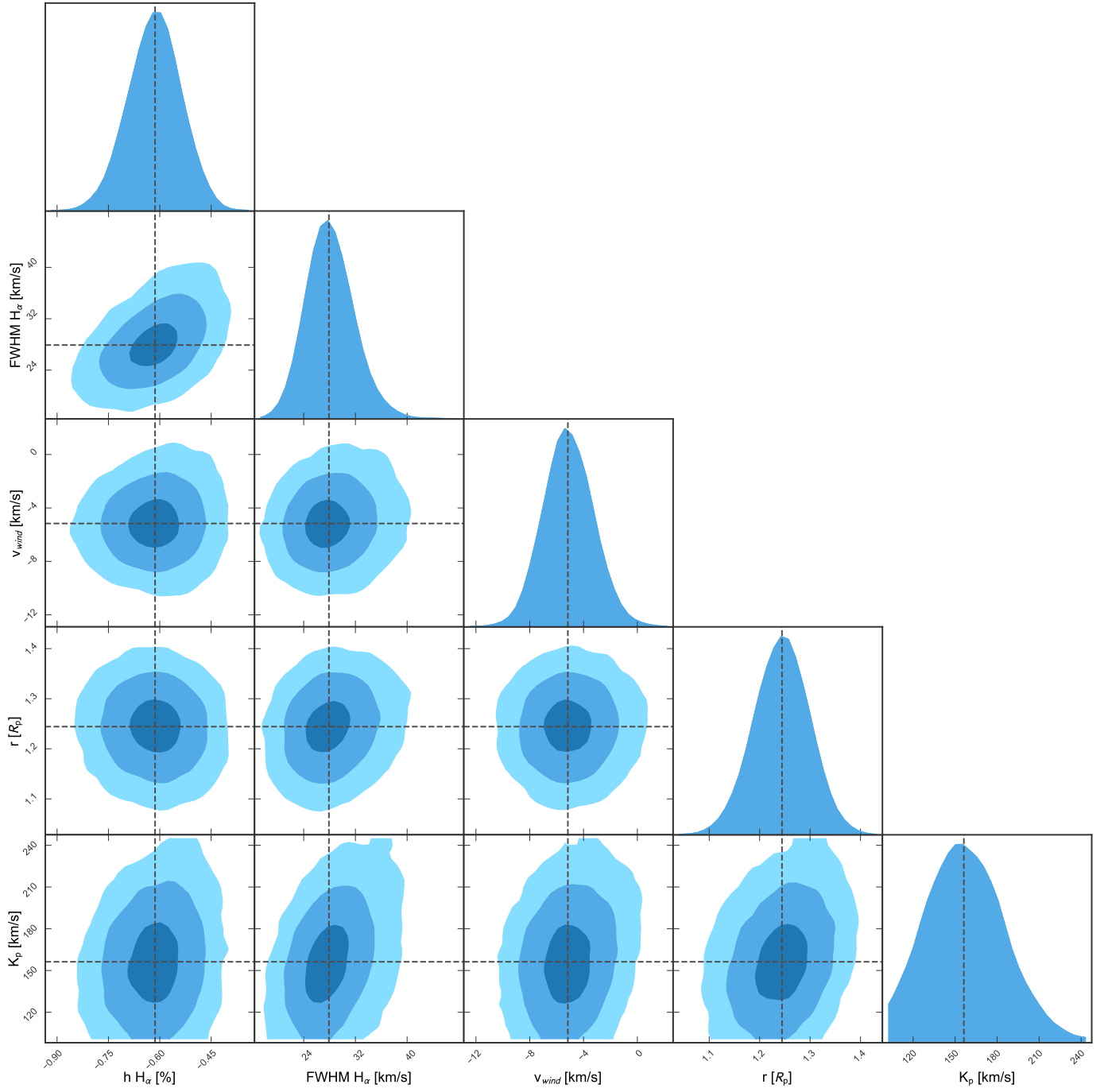
Fig. B.5: Corner plot of MCMC analysis of the \text{H}_\alpha line for KELT-20 b.
