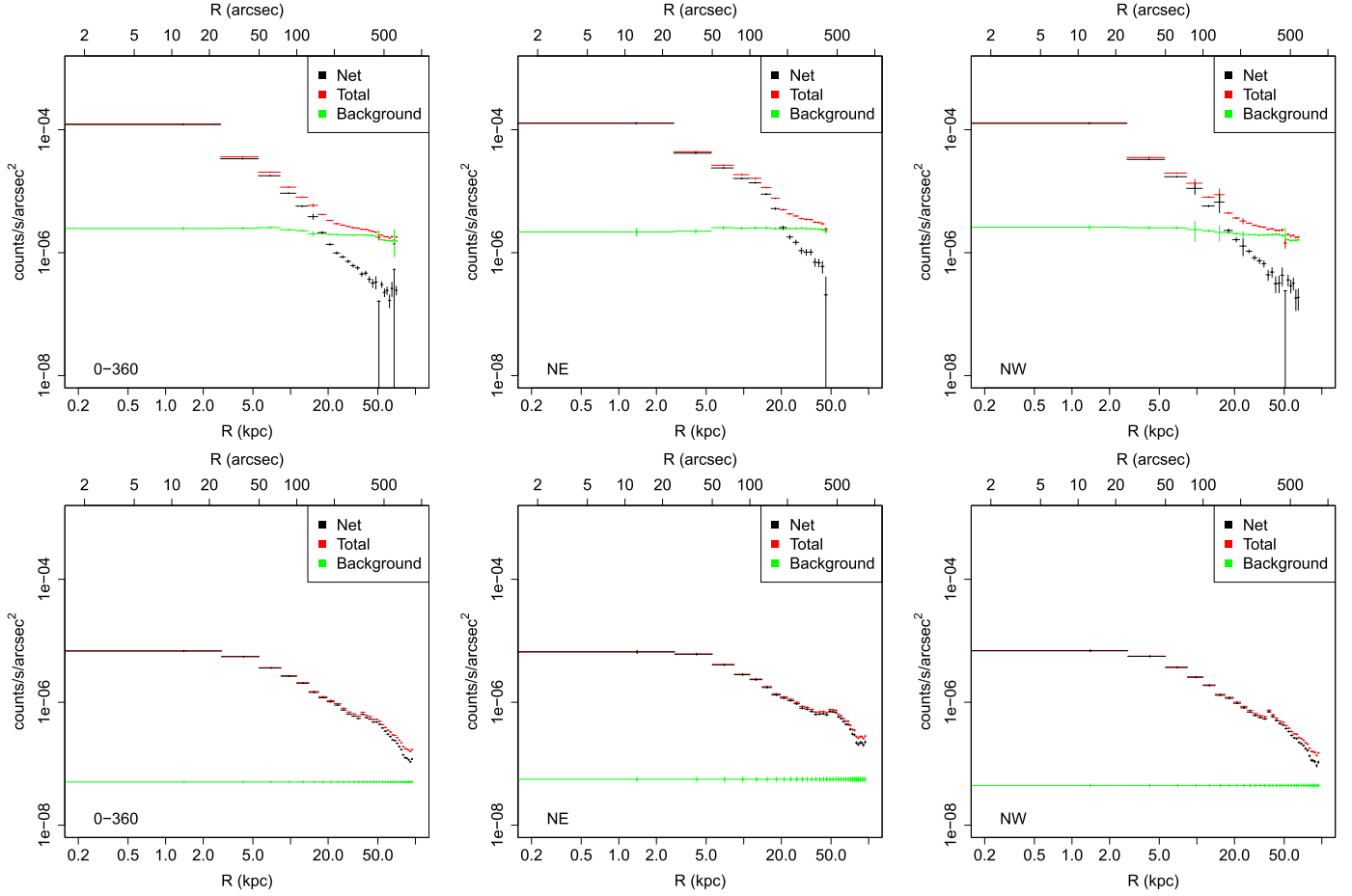
Figure 6. Brightness profiles for NGC 5846 in the 0.3–10 keV band in the different sectors shown in Figure 4, for (from left to right) full (0–360), NE (30–90), and NW (250–30), respectively. In particular, we show brightness profiles for Chandra ACIS data in the top row and for the XMM-MOS data obtained from the reduction procedure proposed by Nevalainen et al. (2005) in the bottom row. The annuli width is \sim 25'' , 50 pixels for Chandra ACIS data and 500 pixels for XMM-MOS data. Red, black, and green points represent total, net, and background brightness profiles, respectively.
