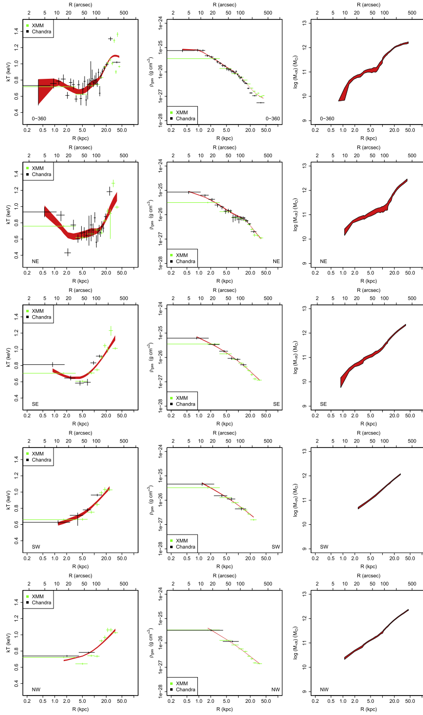
Figure 16. Effect on the X-ray mass profiles of the different sectors selected for the spectral extraction. From left to right we present the gas temperature, gas density, and resulting mass profile for NGC 5846 (with a smoothing parameter of 0.7), while from top to bottom we show the results in the full (0–360), NE (30–90), SE (90–180), SW (180–250), and NW (250–30) sectors, respectively. The minimum signal-to-noise ratio is 30 for XMM-Newton data in all sectors, while for Chandra data the minimum signal-to-noise ratio is 50 in the full (0–360), SW (180–250), and NW (250–30) sectors and 30 in the NE (30–90) and SE (90–180) sectors.
