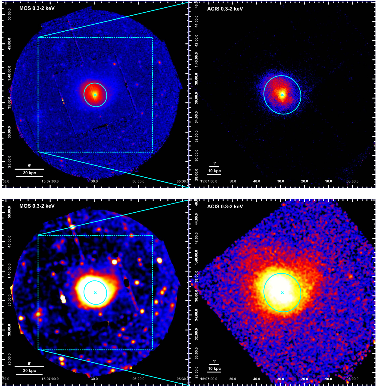
Figure 5. Same as Figure 4, but in the 0.3–2 keV band with the D25 ellipse shown in cyan. Small-scale and large-scale structures are shown in the top and bottom panels, respectively.
