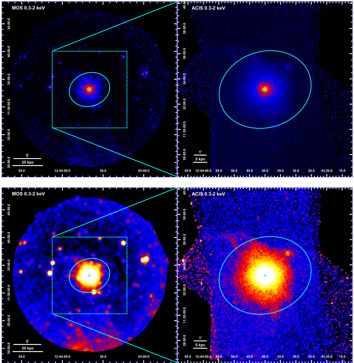
Figure 2. Same as Figure 1, but in the 0.3–2 keV band, with the D25 ellipse shown in cyan. Small-scale and large-scale structures are shown in top and bottom panels, respectively.
