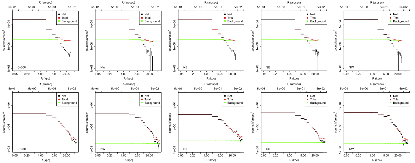
Figure 19. Brightness profiles for NGC 4649 in the 0.3–10 keV band in the different sectors shown in Figure 1, for (from left to right) full (0–360), NW (270–360), NE (90–180), SE (90–180), and SW (180–270), respectively. In particular, we show brightness profiles for Chandra ACIS data in the top row and for the XMM-MOS data obtained from the reduction procedure proposed by Nevalainen et al. (2005) in the bottom row. The annuli width is \sim 25'' , 50 pixels for Chandra ACIS data and 500 pixels for XMM-MOS data. Red, black, and green points represent total, net, and background brightness profiles, respectively.
