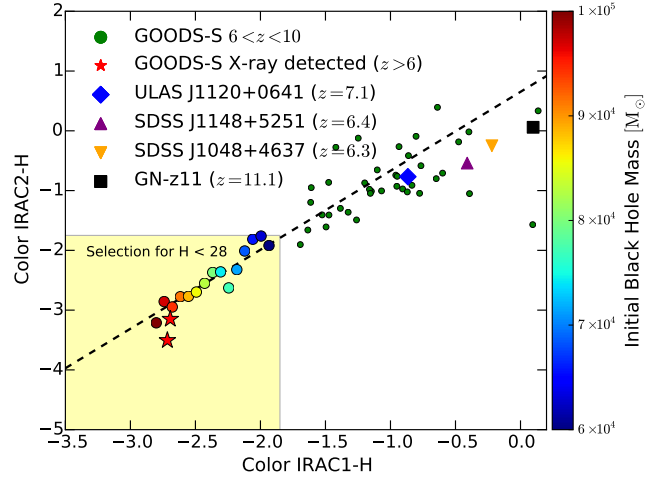
Figure 4. Color-color diagram for objects at z \gtrsim 6 . The yellow-shaded area indicates the region in the diagram where we expect SEDs compatible with the ones predicted for DCBHs, and observable with current surveys. Green points are GOODS-S objects without an X-ray counterpart, while red stars are GOODS-S objects detected in the X-ray and likely powered by accretion onto a collapsed object. Filled circles are, as in Fig. 1, DCBH simulations. In addition, we report the position in the color-color plot of several z > 6 sources. ULAS J1120+0641 (Mortlock et al. 2011; Barnett et al. 2015) is the most distant known QSO ( z \approx 7.1 ). SDSS J1148+5251 (Fan et al. 2003) and SDSS J1048+4637 (Maiolino et al. 2004) are two highly-obscured and dusty QSOs at z \approx 6.4 and z \approx 6.3 , respectively. GN-z11 (Oesch et al. 2016) is the highest redshift galaxy discovered to date ( z \approx 11.1 ).
