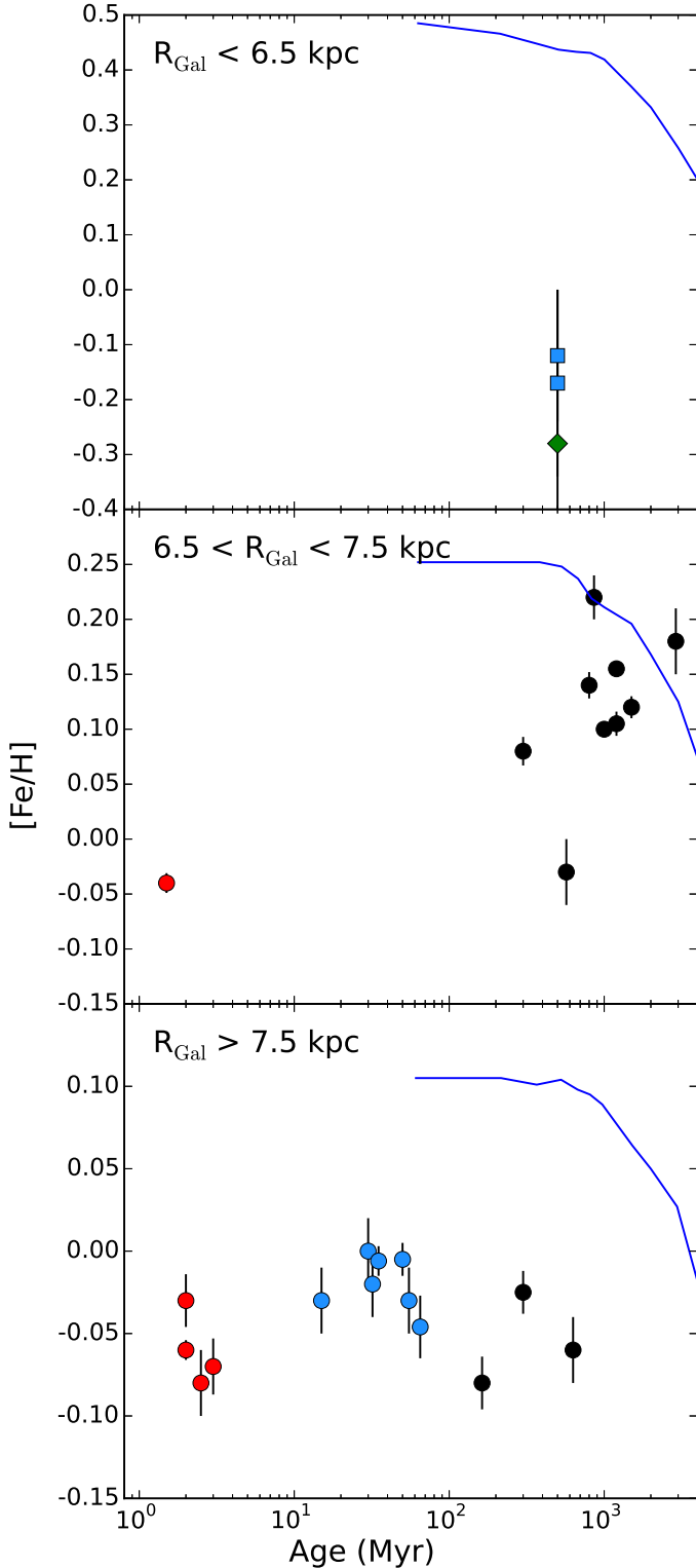
Fig. 9. [Fe/H] variation with age at different Galactic radii. The clusters observed by the Gaia -ESO Survey and the model of Minchev et al. (2014) are represented. The colour code is the same as Fig. 8.
