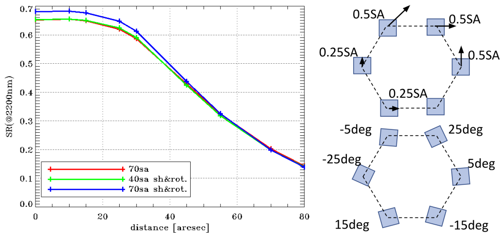
(a) K band SR as a function of the off-axis angle for different LGS WFSs configurations. (b) Shifts and rotations scheme.
