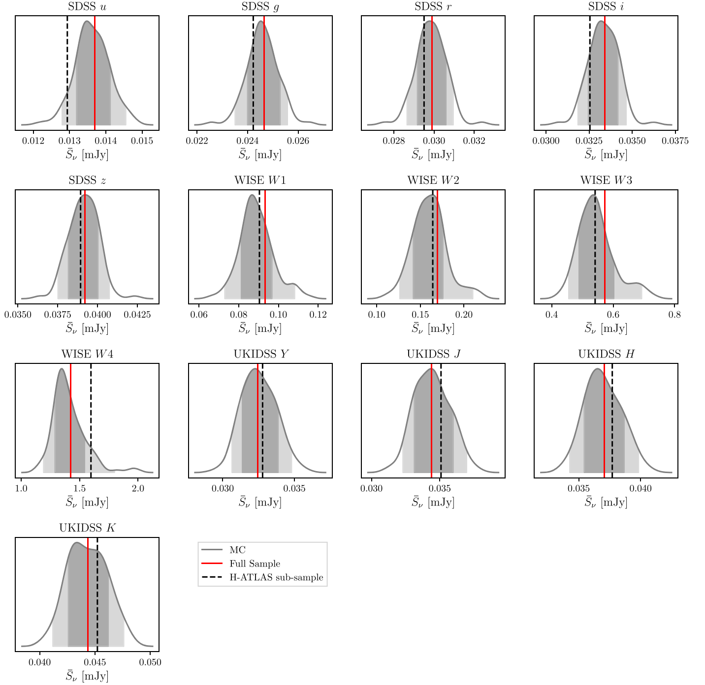
Figure 8. Assessment of the H-ATLAS subsample representativity. In each panel, the gray line shows a kernel density estimate of the distribution of the mean fluxes in a certain photometric band estimated from a set of 100 random subsamples. The darker and lighter shaded areas indicate the \pm 1\sigma and \pm 2\sigma of the average flux distribution, evaluated as the (13.6, 86.4) and (2.1, 97.9) percentiles of the distribution, respectively. The solid red and dashed black lines denote the average flux measured for whole QSO sample and the H-ATLAS subsample, respectively.
