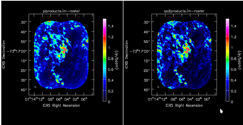
Figure 3. N83C (CO)
