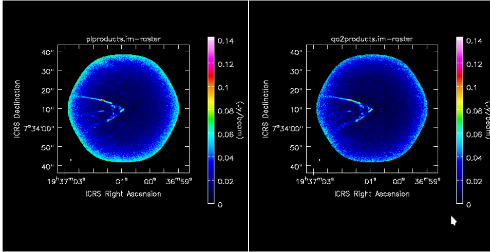
Figure 2. B335 (CO 2-1)
