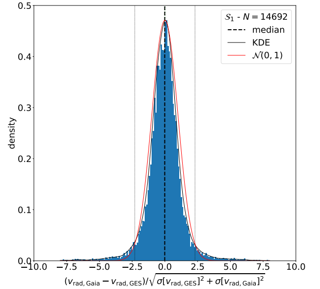
Fig. 7: Probability distribution of the normalised velocity differences. The blue histogram (bin width = 0.1) displays the distribution \Delta_{\text{norm}} v_{\text{rad}} of the difference of the radial velocity differences v_{\text{rad,Gaia}} - v_{\text{rad,GES}} normalised by the propagated errors \sqrt{\sigma[v_{\text{rad,Gaia}}]^2 + \sigma[v_{\text{rad,GES}}]^2} . The black line is the empirical KDE obtained from the sample distribution. The red line is the probability distribution function (PDF) of a the normal law centred in 0 and of unit variance. The dashed vertical black line indicates the mean of the distribution. The black dotted lines have equation |\Delta_{\text{norm}} v_{\text{rad}}| = 2.3 and show where the tails of the empirical distribution become heavier than those of the normal law.
