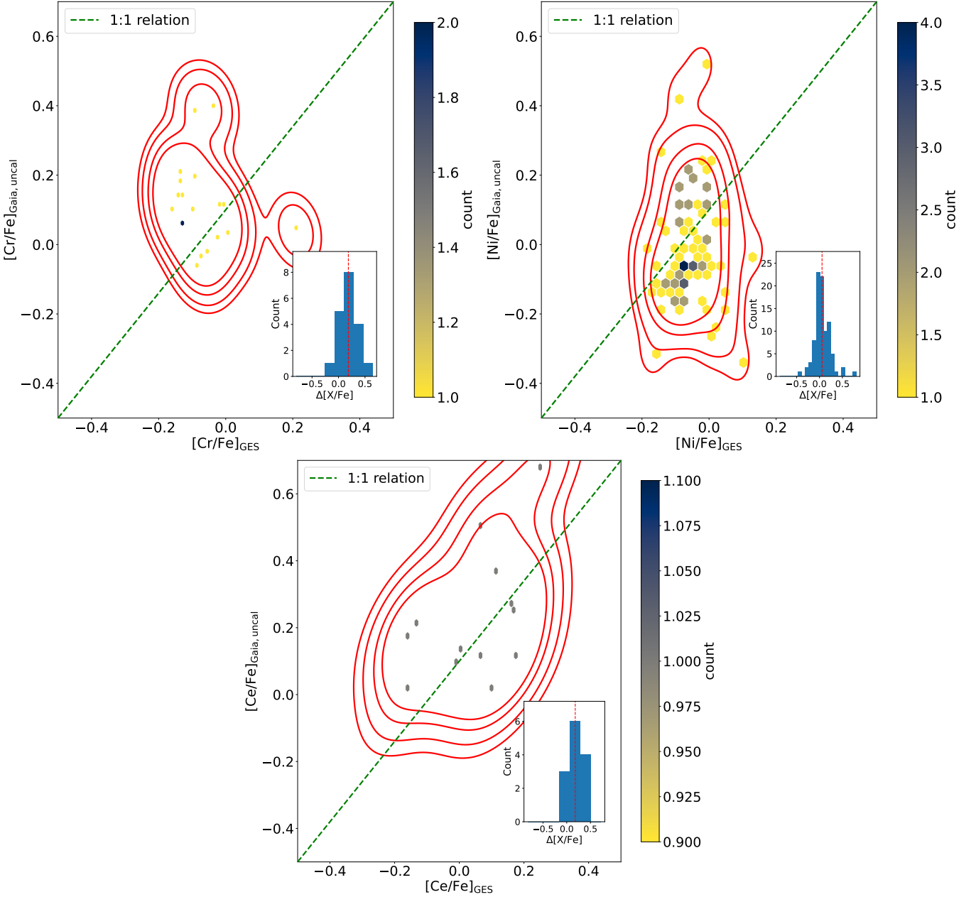
Fig. 18: Comparison of the Gaia -ESO [X/Fe] with the Gaia uncalibrated [X/Fe] for the following chemical species (from top to bottom, left to right): Cr, Ni, and Ce. Symbols and colours are as in the Fig. 11.
