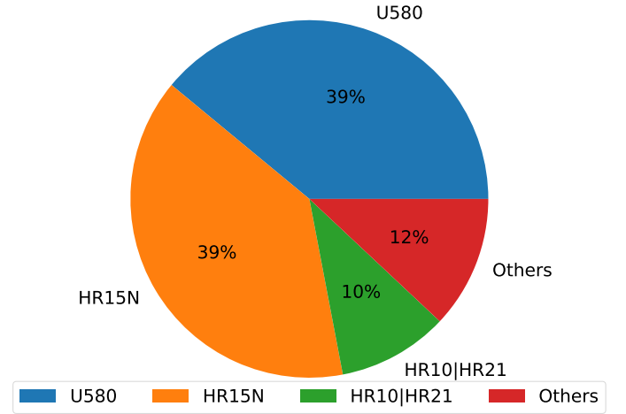
Fig. 5: Pie chart of the distribution of the 2079 stars of the subsample S_3 according to the GES setup used to derive the GES recommended atmospheric parameters.
