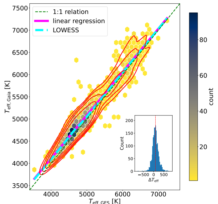
Fig. 11: Comparison of the effective temperatures for the 1939 stars of S_3 with both a Gaia GSP-Spec and GES temperature estimate. The 2D hexagonal bins are colour-coded by the number of stars. The red lines show density levels containing 68, 80, 90 and 95 % of the population. The dashed green line shows the 1-to-1 relation, the pink thick line is the linear regression (see text for the parametrisation). The cyan thick dashed line is the LOWESS line. The inset shows the distribution of \Delta T_{\text{eff}} = T_{\text{eff,Gaia}} - T_{\text{eff,GES}} .
