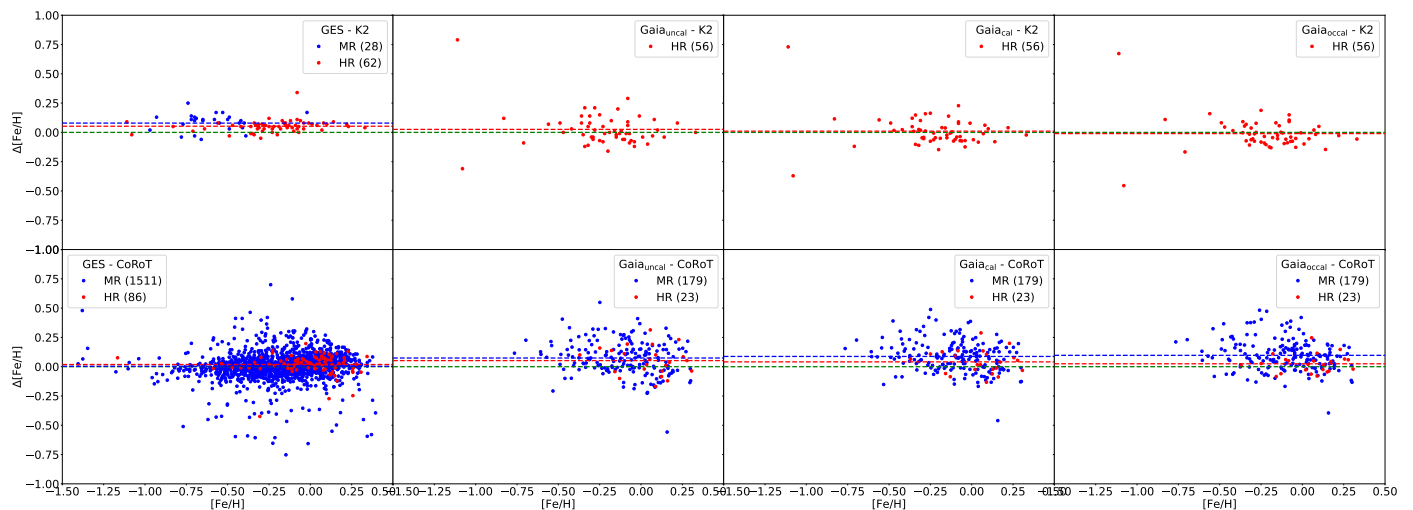
Fig. 24: Comparison of [\text{Fe}/\text{H}] values as a difference to the reference seismic values (K2 or CoRoT) for Gaia -ESO, Gaia , Gaia calibrated, and Gaia OC-calibrated. Top row: comparison with K2; bottom row: comparison with CoRoT. The HR (red) and MR (blue) reference samples are shown.
