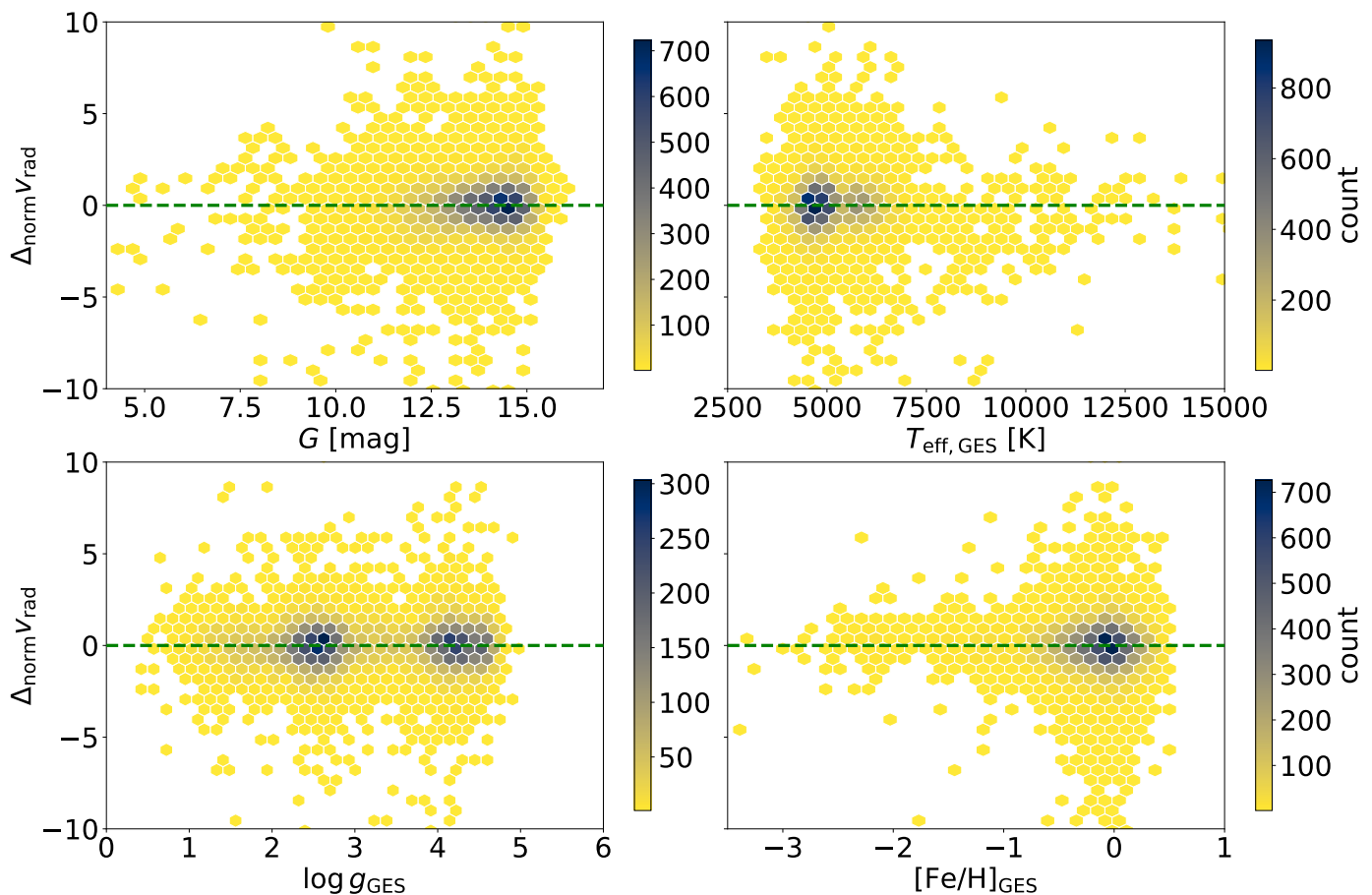
Fig. 8: From top to bottom, left to right: \Delta_{\text{norm}} V_{\text{rad}} vs. G magnitude, T_{\text{eff,GES}} , \log g_{\text{GES}} and [\text{Fe}/\text{H}]_{\text{GES}} . The vertical axis is the same for the four panels. The colour scale changes from one plot to another.
