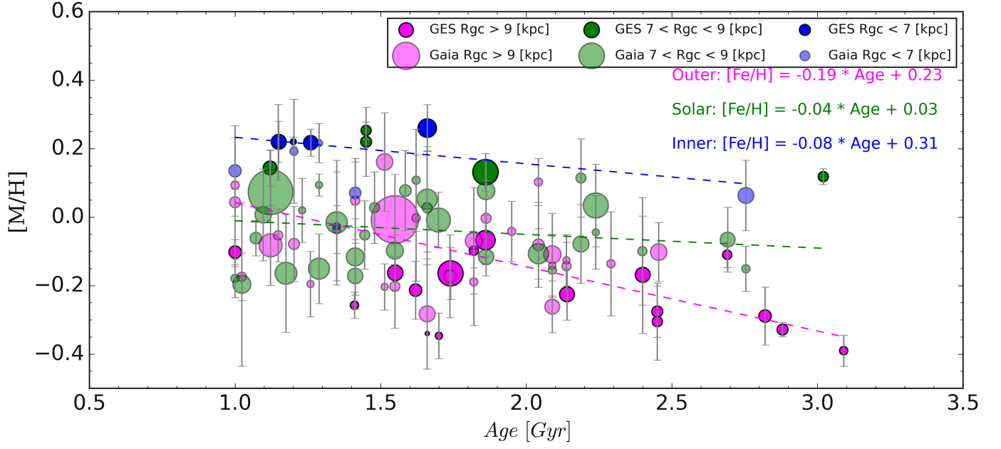
Fig. 31: Age-Metallicity relation for the sample of clusters with ages between 1 and 3 Gy, divided in three radial bins. The clusters observed by Gaia are represented with semi-transparent circles, while those observed by GES with solid-filled circles. The linear regressions are shown with dashed lines using the same colour as the corresponding radial bin. In the plot, we show the coefficients of the three age-metallicity relationships. The size of the symbols is proportional of the number of member stars used to compute the mean values.
