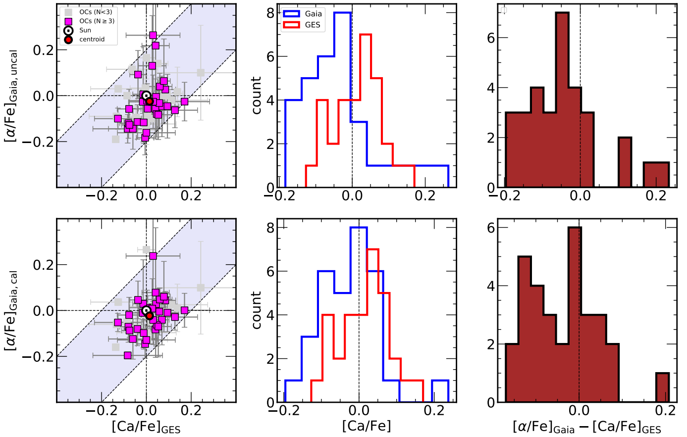
Fig. 29: GES [Ca/Fe] vs. Gaia [\alpha/Fe] (uncalibrated, calibrated) for 52 open clusters in common. Similar panels as in Fig. 28.
