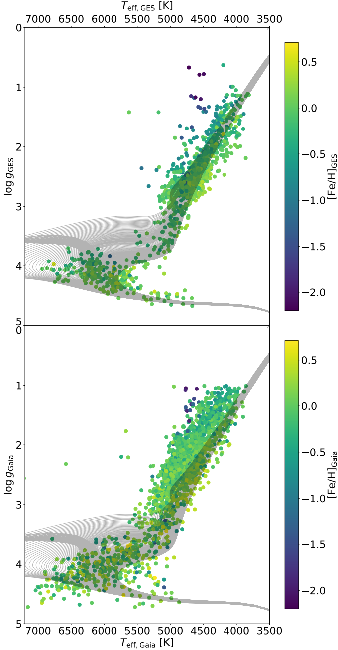
Fig. 3: Kiel diagram of the 2079 stars in the subsample S_3 , colour-coded by metallicity. A grid of Parsec isochrones (Bresnan et al., 2012) with solar metallicity and ages ranging from 0.1 to 14 Gy is superimposed. Top panel: based on the Gaia -ESO atmospheric parameters; bottom panel: based on the uncalibrated Gaia GSP-Spec atmospheric parameters.
