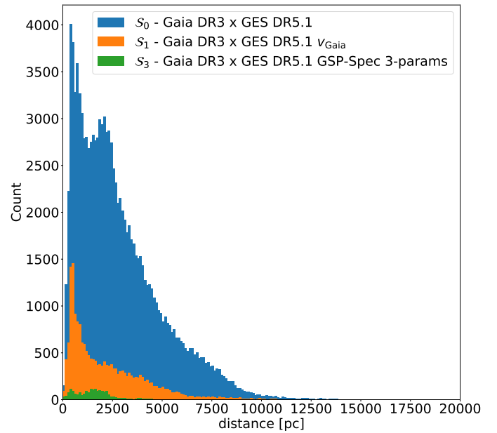
Fig. 2: Distributions of the Gaia distances (Bayesian distances from Bailer-Jones et al., 2021) of the of the GES parent sample ( S_0 ; blue), of the stars having a Gaia DR3 radial velocity ( S_1 ; orange), and of the stars having the three main Gaia GSP-Spec atmospheric parameters ( S_3 ; green). The bin positions and width are identical for the three histograms; the bin width was adjusted using the Freedman-Diaconis rule.
