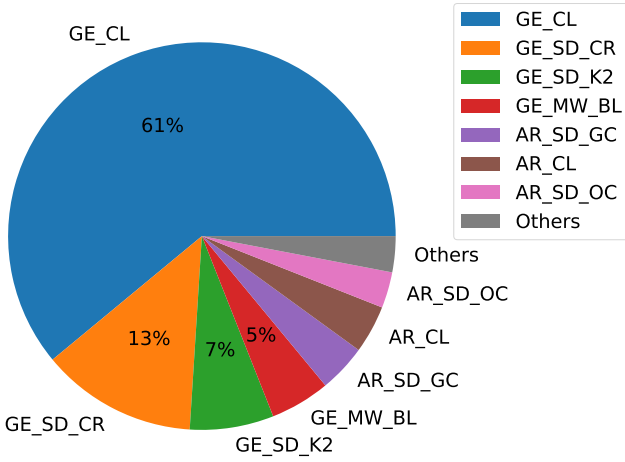
Fig. 6: Pie chart of the distribution of the 2079 stars of the sub-sample S_3 according to their GES field type.
