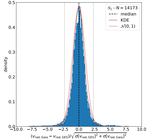
Fig. A.1: Probability distribution of the normalised velocity differences. The blue histogram (bin width = 0.1) displays the distribution \Delta_{\text{norm}} v_{\text{rad}} of the difference of the radial velocity differences v_{\text{rad, Gaia}} - v_{\text{rad, GES}} normalised by the propagated errors \sqrt{\sigma[v_{\text{rad, Gaia}}]^2 + \sigma_{\text{corr}}[v_{\text{rad, GES}}]^2} where \sigma_{\text{corr}}[v_{\text{rad, GES}}] is the uncertainty corrected according to Babusiaux et al. (2023). The black line is the empirical KDE obtained from the sample distribution. The red line is the probability distribution function (PDF) of a the normal law centred in 0 and of unit variance. The dashed vertical black line indicates the mean of the distribution. The black dotted lines have equation |\Delta_{\text{norm}} v_{\text{rad}}| = 2.3 and show where the tails of the empirical distribution become heavier than those of the normal law.
