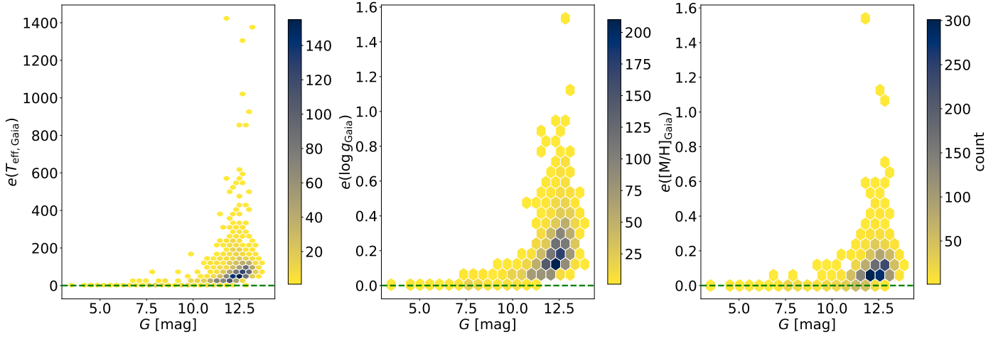
Fig. 21: Correlation between e(\mathcal{P}_{\text{Gaia}}) and G where \mathcal{P} is either T_{\text{eff}} , \log g or [M/H] (from left to right).
