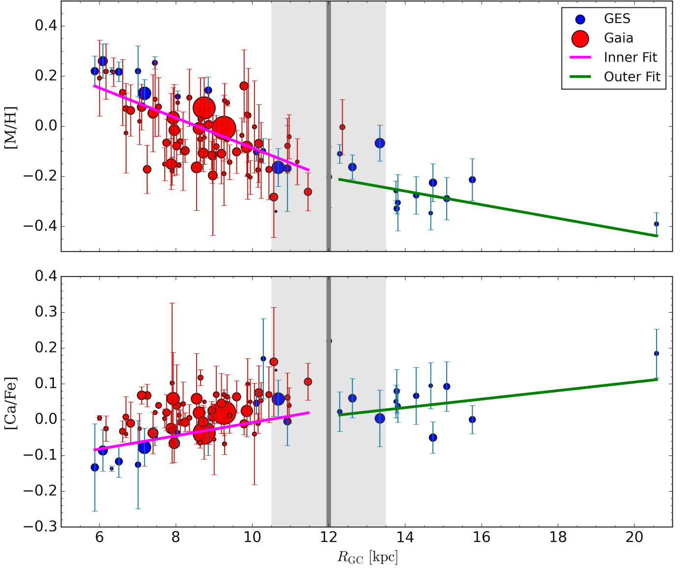
Fig. 30: Metallicity and [Ca/Fe] as a function of the Galactocentric radius for the sample of Gaia and GES open clusters with 1 \text{ Gy} < \text{age} < 3 \text{ Gy} . In the upper panel, we show [M/H] (calibrated metallicity for Gaia and [Fe/H] for GES) as a function of R_{GC} , while in the bottom panel, we present [Ca/Fe] versus R_{GC} . The weighted linear fits are shown with continuous lines. The vertical line mark the location of the ELBOW. The size of the symbols is proportional of the number of member stars used to compute the mean values.
