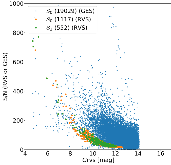
Fig. A.3: GES S/N and RVS S/N as a function of G for respectively 19029 (blue) and 1117 (orange) objects of S_0 with a valid GES (resp., RVS) S/N and RVS S/N as a function of G for the 552 (green) objects of S_3 with a valid RVS S/N.
