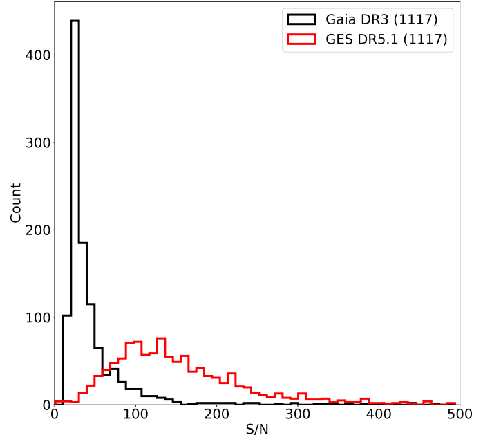
Fig. 4: Distributions of the GES (red) and Gaia RVS (black) S/N for 1117 stars having both values.
