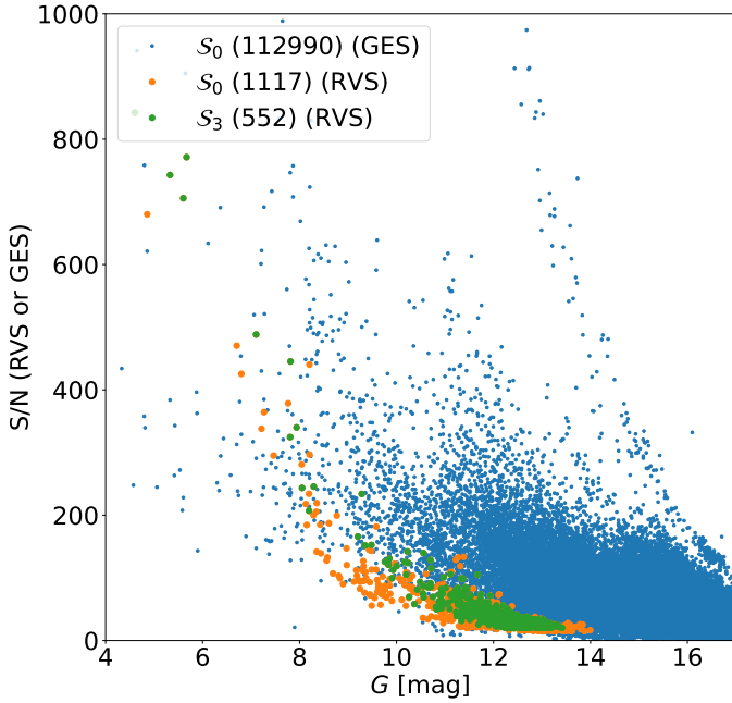
Fig. 22: GES S/N and RVS S/N as a function of G for respectively 112990 (blue) and 1117 (orange) objects of S_0 with a valid GES (resp., RVS) S/N and RVS S/N as a function of G for the 552 (green) objects of S_3 with a valid RVS S/N.
