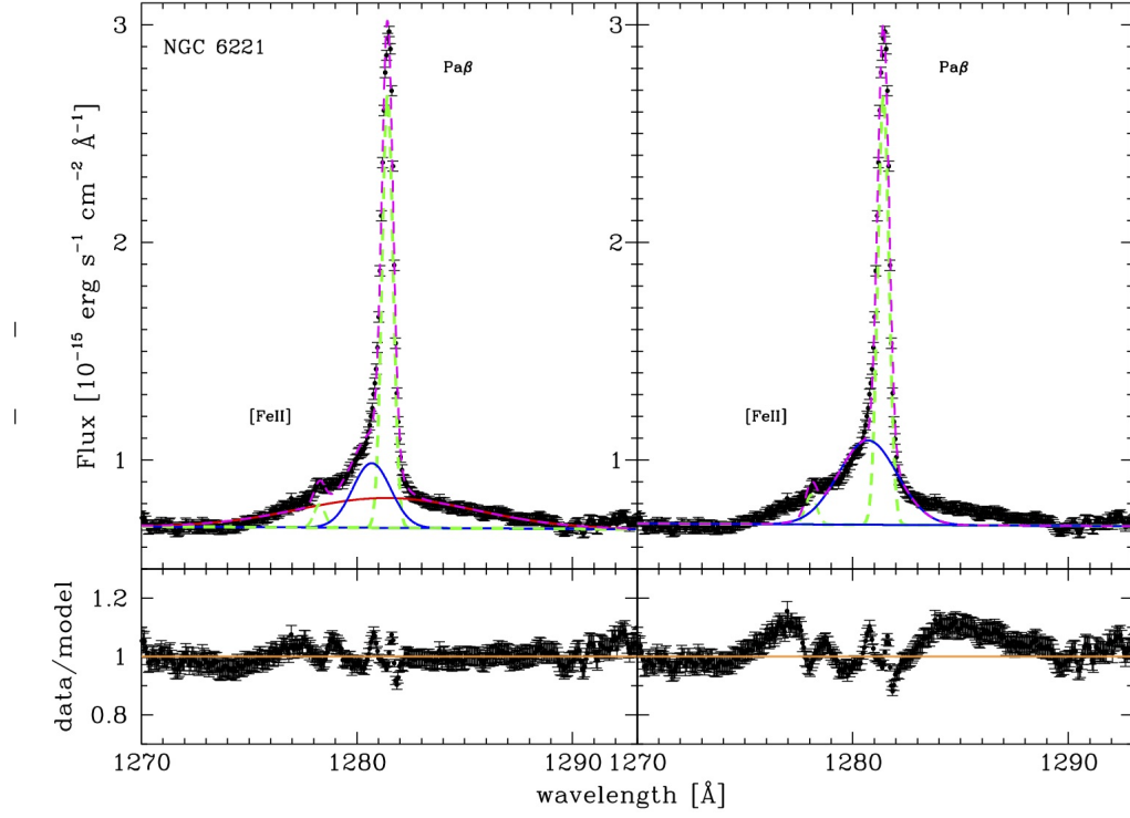
Figure A8. Left: Best fit of the Pa \beta line of NGC 6221 including a broad (FWHM = 2257 \text{ km s}^{-1} ) component. Right: Same as before without including a broad Pa \beta component. Lower panels show the data to model ratio.
