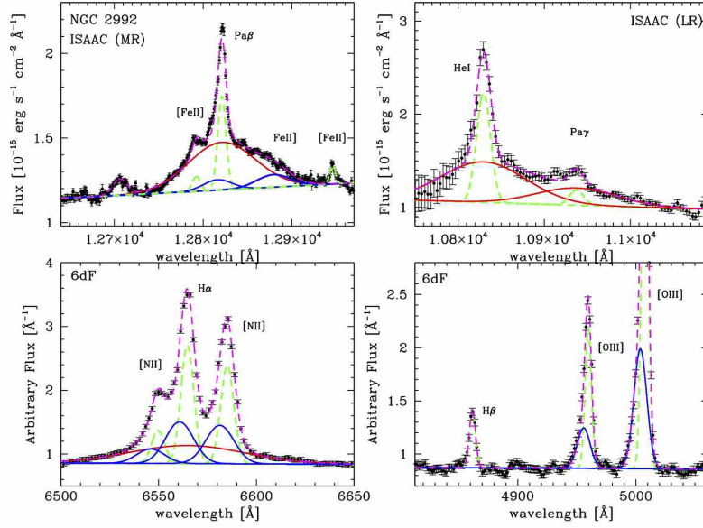
Figure 15. Near infrared and optical spectra of NGC 2992, corrected for redshift. Top-left: Pa \beta + [\text{Fe II}] region. Top-right: He I+Pa \gamma region. Bottom-left: H \alpha + [\text{N II}] region. Bottom-right: H \beta + [\text{O III}] region. The narrow, intermediate and broad components are shown with green-dashed, blue and red lines, respectively. The magenta-dashed line shows the total fitting model.
