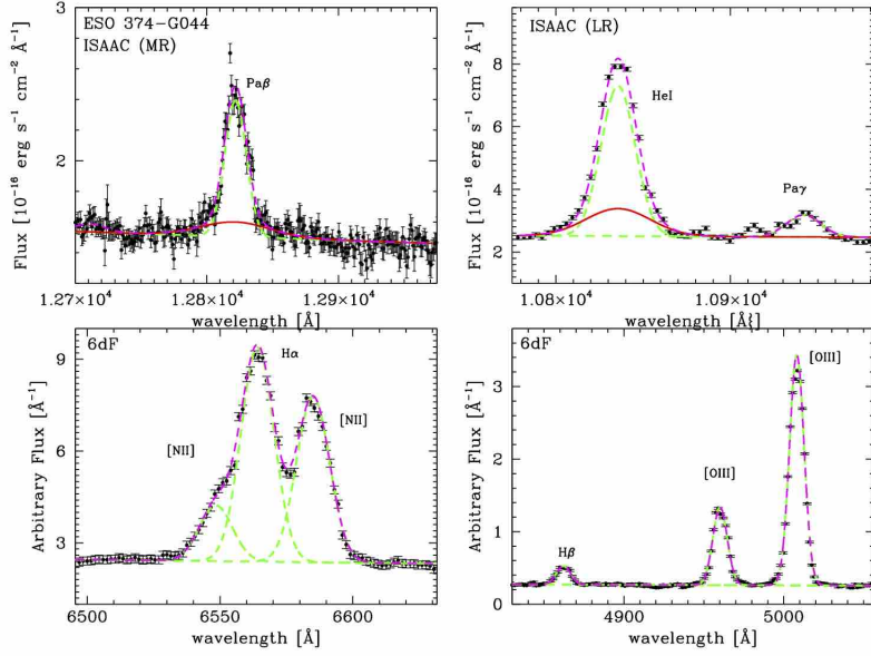
Figure 9. Near infrared and optical spectra of ESO 374-G044, corrected for redshift. Top-left: Pa \beta +Fe II region. Top-right: He I+Pa \gamma region. Bottom-left: H \alpha +N II region. Bottom-right: H \beta +O III region. The narrow, intermediate and broad components are shown with green-dashed, blue and red lines, respectively. The magenta-dashed line shows the total fitting model.
