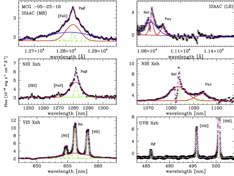
Figure 11. Near infrared and optical spectra of MCG -05-23-016, corrected for redshift. Top-left: ISAAC MR Pa \beta + [\text{Fe II}] region. Top-right: ISAAC LR He I+Pa \gamma region. Center-left: X-shooter Pa \beta + [\text{Fe II}] region. Center-right: X-shooter He I+Pa \gamma region. Bottom-left: X-shooter H \alpha + [\text{N II}] region. Bottom-right: X-shooter H \beta + [\text{O III}] region. The narrow, intermediate and broad components are shown with green-dashed, blue and red lines, respectively. The magenta-dashed line shows the total fitting model.
