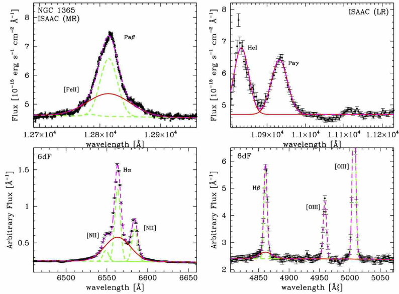
Figure 14. Near infrared and optical spectra of NGC 1365, corrected for redshift. Top-left: Pa \beta region. Top-right: He I+Pa \gamma region. Bottom-left: H \alpha +N II region. Bottom-right: H \beta +O III region. The narrow, intermediate and broad components are shown with green-dashed, blue and red lines, respectively. The magenta-dashed line shows the total fitting model.
