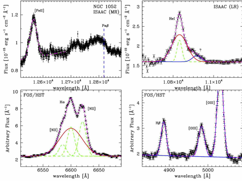
Figure 13. Near infrared and optical spectra of NGC 1052, corrected for redshift. Top-left: Pa \beta +Fe II region. Top-right: He I+Pa \gamma region. Bottom-left: H \alpha +N II region. Bottom-right: H \beta +O III region. The narrow, intermediate and broad components are shown with green-dashed, blue and red lines, respectively. The magenta-dashed line shows the total fitting model. The blue-dashed vertical line indicate the Pa \beta position.
