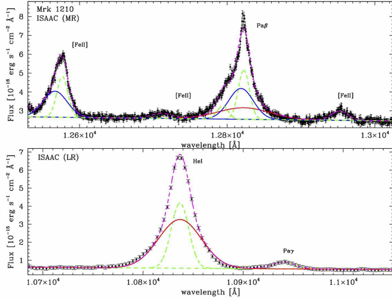
Figure 12. Near infrared spectrum of Mrk 1210, corrected for redshift. Top: Pa \beta + [\text{Fe II}] region. Bottom: He I+Pa \gamma region. The narrow, intermediate and broad components are shown with green-dashed, blue and red lines, respectively. The magenta-dashed line shows the total fitting model.
