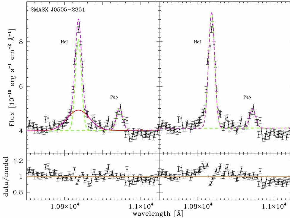
Figure A1. Left: Best fit of the He I and Paγ lines of 2MASX J0505–2351 including the broad (FWHM = 1736 km s −1 ) He I component. Right: Same as before without including the broad He I component. Lower panels show the data to model ratio.
