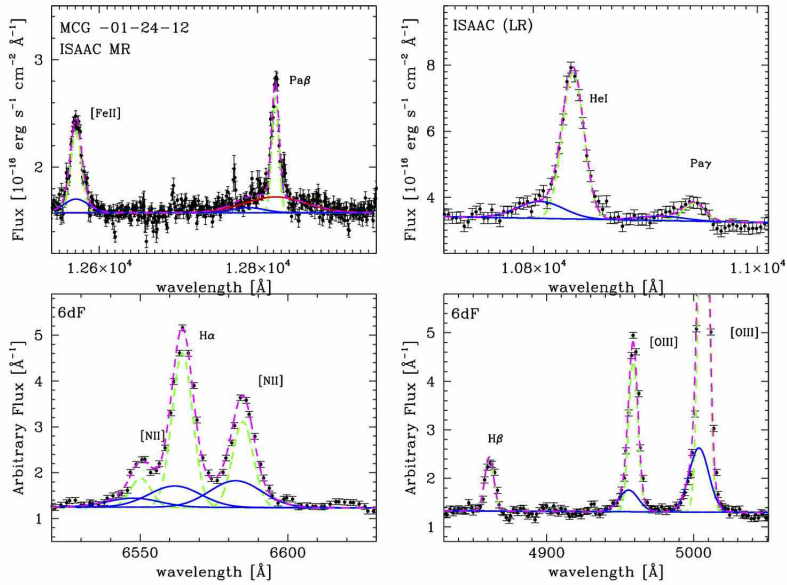
Figure 10. Near infrared and optical spectra of MCG -01-24-012, corrected for redshift (see also La Franca et al. 2015 ). Top-left: Pa \beta +Fe II region. Top-right: He I+Pa \gamma region. Bottom-left: H \alpha +N II region. Bottom-right: H \beta +O III region. The narrow, intermediate and broad components are shown with green-dashed, blue and red lines, respectively. The magenta-dashed line shows the total fitting model.
