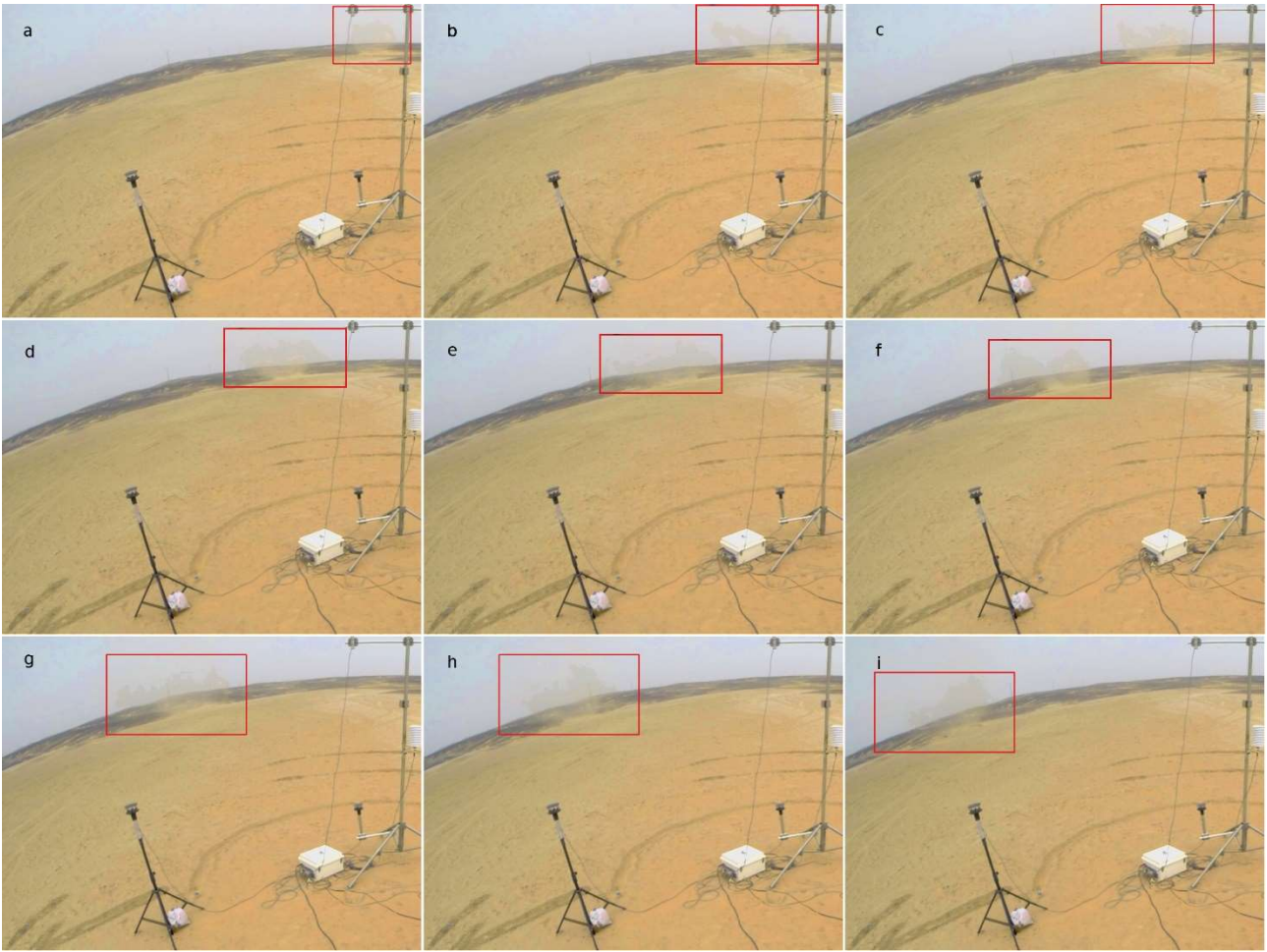
476 Fig. 12 The dust devil of Fig. 11 during its passage at ~ 61 m from the station.
