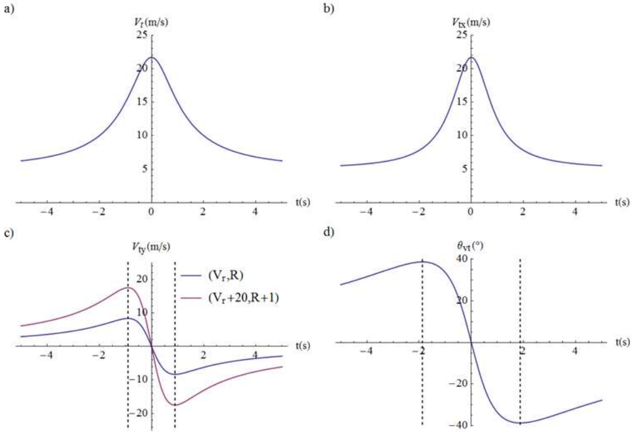
Fig. 5 Wind speed signatures of a dust devil concordantly rotating as seen by a fixed meteorological station. The event in blue has the following parameters: s = 5 \text{ m/s} , \theta_s = 0 , V_r = 25 \text{ m/s} , R = 3 \text{ m} , d_o = 4.5 \text{ m} . The four plots are:
