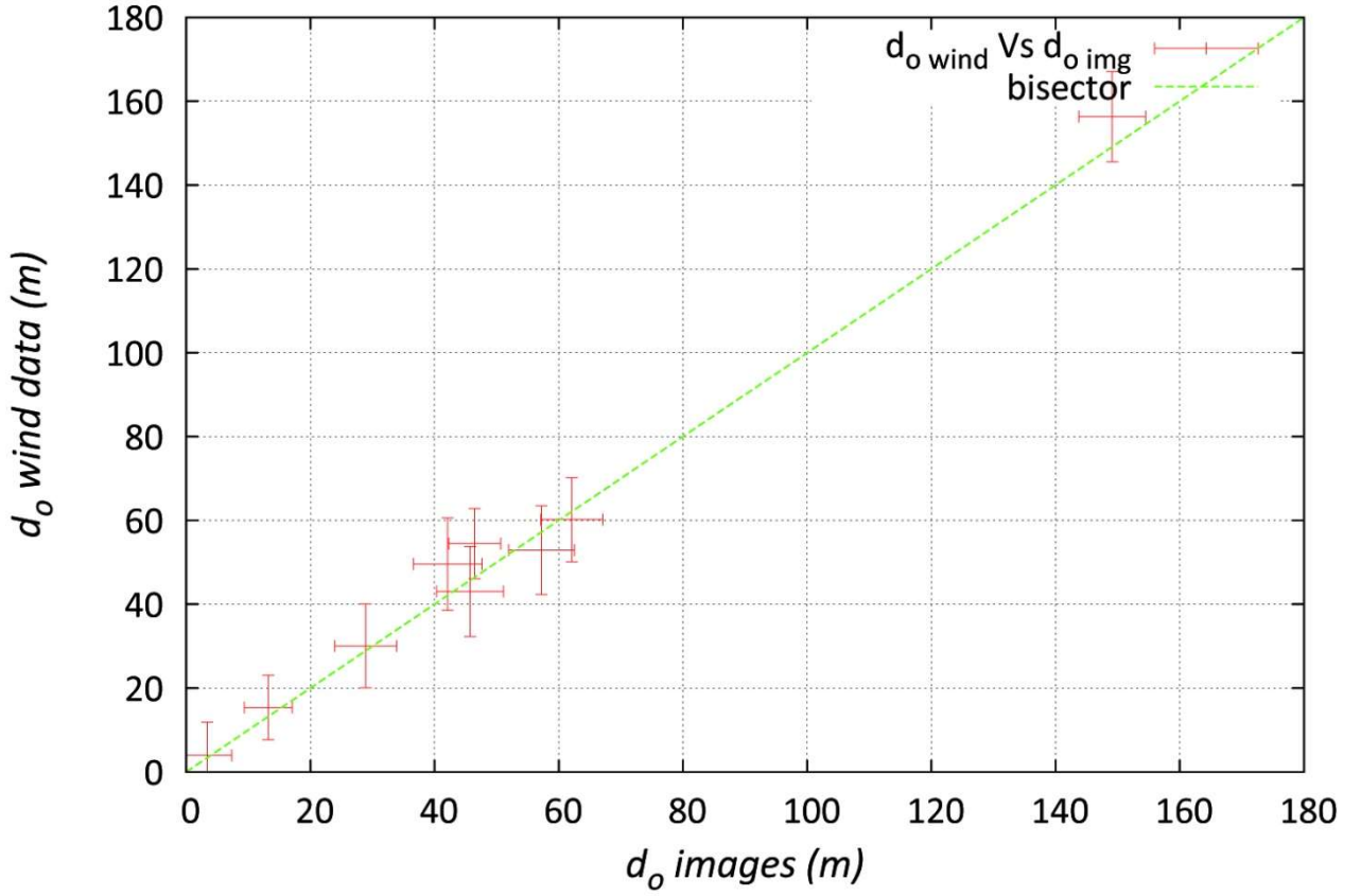
Fig. 16 The impact parameters d_o obtained from the images on x axis, compared with the ones obtained by the study of the wind speed signal. All points are compatible within uncertainties with the bisector, proving the agreement of the two methods.
