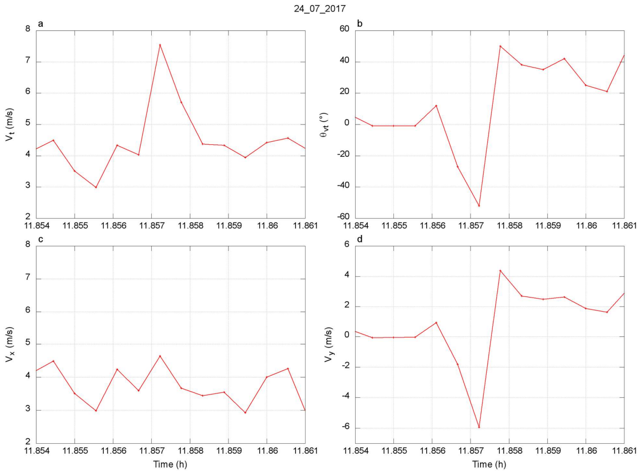
499 500 Fig. 15 The wind speed and direction signature of one of the passing dust devil. Fig. a) shows the total wind speed v_t (the direct 501 measure of the anemometer); b) the direction of the vector v_t already normalized to zero mean; c) the x-projection of v_t (where 502 x is the direction of the translational motion of the vortex); d) the y-projection of v_t . In the b and d plots the minimum of the 503 signature precedes the maximum and this indicates that the vortex rotates discordantly to its translational motion. 504
