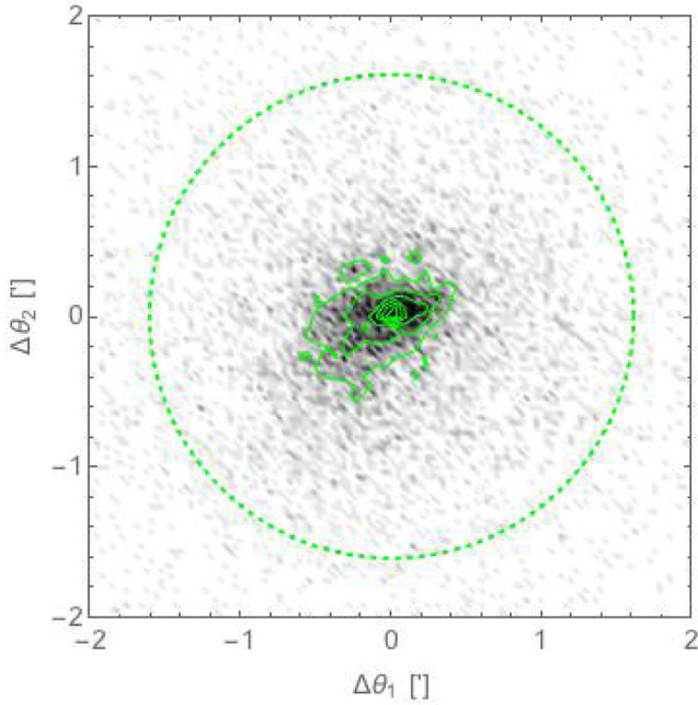
Figure 2. Chandra exposure-corrected image in the [0.7–2] keV band used for the spatial analysis. The dashed green circle of radius \theta_{80\text{ per cent}} = 1.61 arcmin encloses 80 per cent of the source light. Green contours are X-ray SB contours at arbitrary levels. The image is centred on the optical centre. North is top and east is left.
