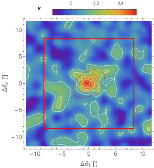
Figure 9. Two-dimensional WL mass map of MACS1206 reconstructed using wide-field multi-colour imaging observations. The image is 24\text{ arcmin} \times 24\text{ arcmin} in size and centred on the optical cluster centre. For visualization purposes, the image was smoothed with a Gaussian kernel of standard deviation 1.5\text{ arcmin} . The colour bar indicates the lensing convergence \kappa for a reference source at z_s = 20000 . The convergence isopleths go from \kappa = 0.1 to 1.0 , with increments of 0.1 . White and red contours follow the smoothed map and the predicted median NFW profile obtained assuming a flat prior for the axial ratio q_{\text{mat},1} of the matter distribution and q_{\text{ICM}} \geq q , respectively. The red square of semi-size 2\text{ Mpc } h^{-1} \sim 8.39\text{ arcmin} encloses the WL region used for inference. North is top and east is left.
