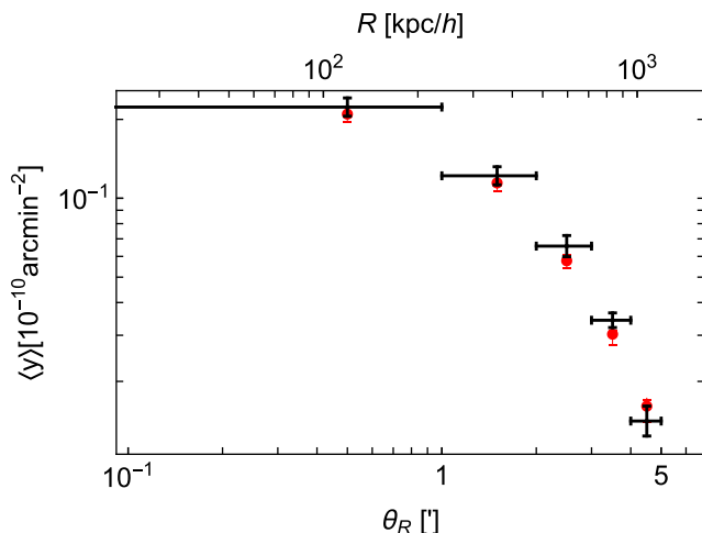
Figure 6. Mean Compton parameter in circular annuli. Black points denote the combined Bolocam/Planck data, and the horizontal black bars cover the radial range of the annulus. Red points and bars denote the median fitted values obtained assuming a flat prior for the axial ratio q_{\text{mat},1} of the matter distribution and q_{\text{ICM}} \geq q . The plotted lines stem from the combined fit to all probes.
