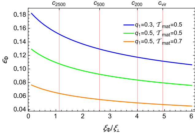
Figure B2. Projected ellipticity of the isopotential surfaces of an NFW halo with c_{200} = 4 as a function of the elliptical radius. The orientation of the halo is fixed by \cos \vartheta = 0.5 and \phi = \pi/3 .
