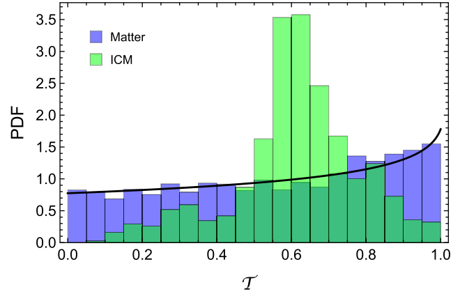
Figure 20. Marginalized PDFs (plotted as histograms) of the triaxial parameter \tau of the total matter (blue) and of the gas distribution (green). The regression assumed a flat prior for the axial ratio q_{\text{mat},1} of the matter distribution and q_{\text{ICM}} \geq q . The black line shows the prior.
