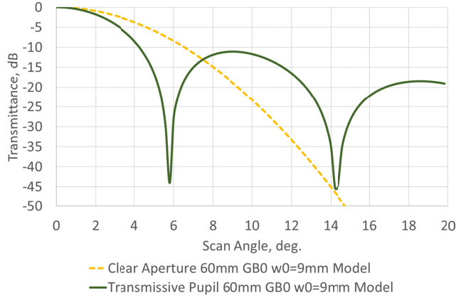
Fig. 4. Analysis of the equivalent transmissive pupil using the analytical model, Eq. (2), with the inner pattern diameter of 15mm, outer device diameter of 60 mm and Gaussian beam waist of 9 mm, see Fig. 5(a). The inner coronae dimensions are the same as those in Fig. 2. The curves are normalized to the respective level at 0°.
