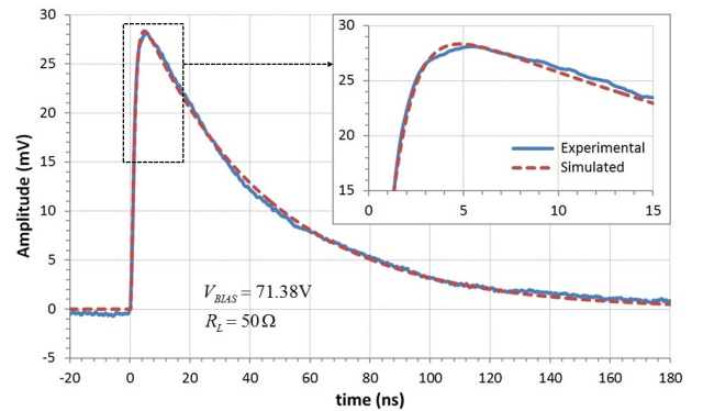
Fig. 8. Simulated and experimental output pulse waveform comparison.
