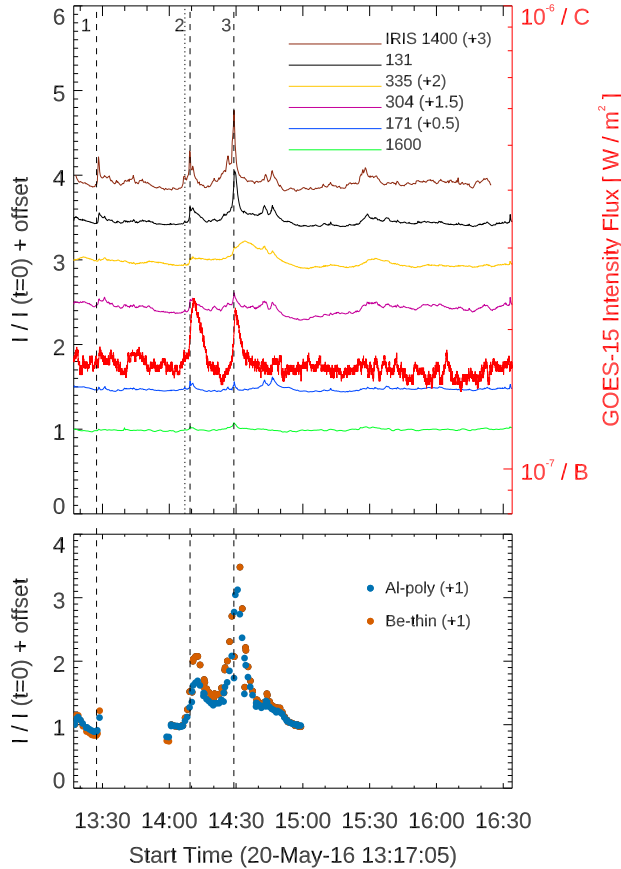
Figure 5. Top panel: Light curves computed from the SDO /AIA observations and IRIS /SJI 1400 Å data obtained on 2016 May 20 from 13:17 UT to 16:30 UT. The red line represents the X-ray flux measured by GOES -15 in the 1 – 8 Å channel. Note the offsets of the light curves along the y direction, to enhance their visibility. The vertical dotted line indicates the starting time of IBIS observations. The three dashed green lines mark the occurrence of the three brightening events E1 , E2 , and E3 , which are described in Sections 3.2 and 3.3 and shown in Figures 6, 7, and 9. Bottom panel: Blue and orange dots represent X-ray light curves obtained from HINODE /XRT data through the Al pol and Be thin filters, respectively.
